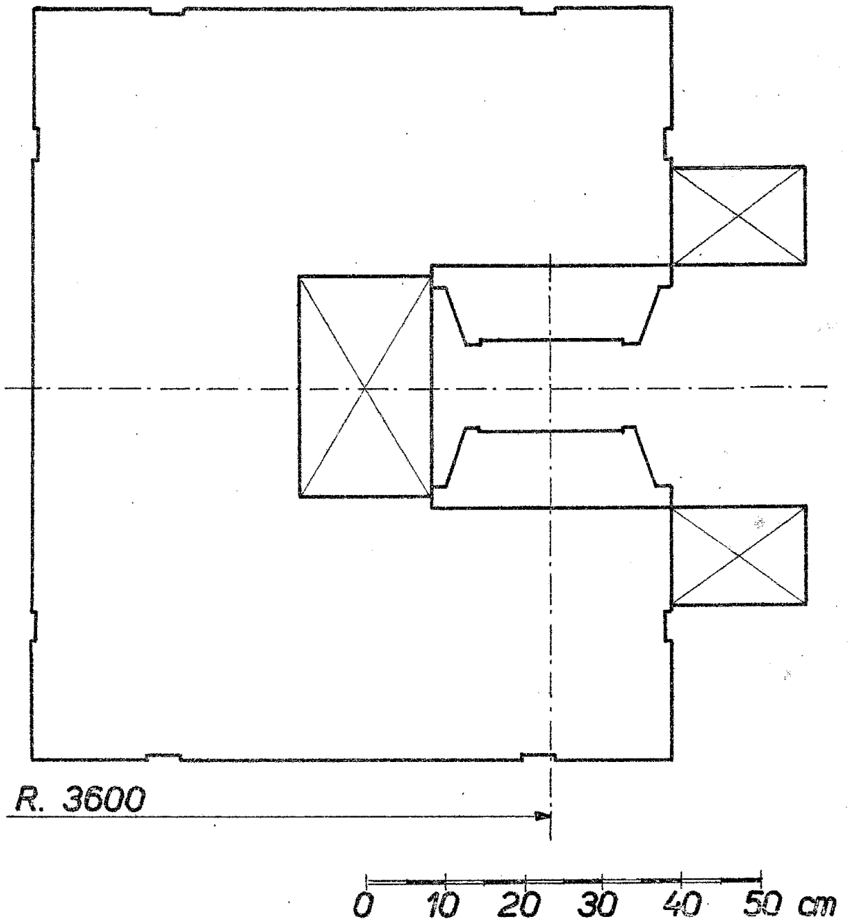
FIG.4 - RADIAL SECTION OF THE MAGNET
