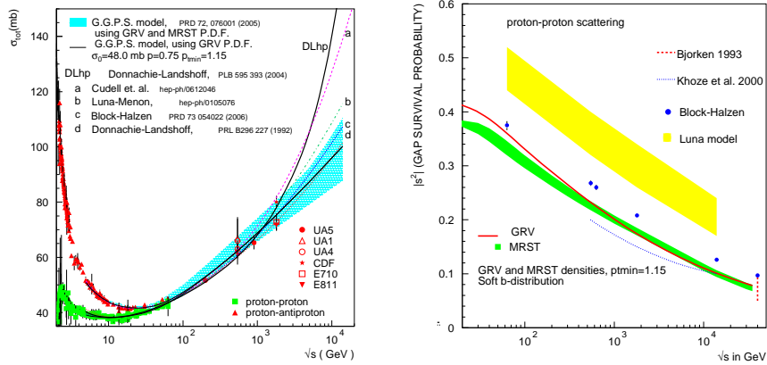
Figure 1: Total cross-section data [8] and models [9](left) and survival probability for large rapidity gaps for different models [10] (right).
