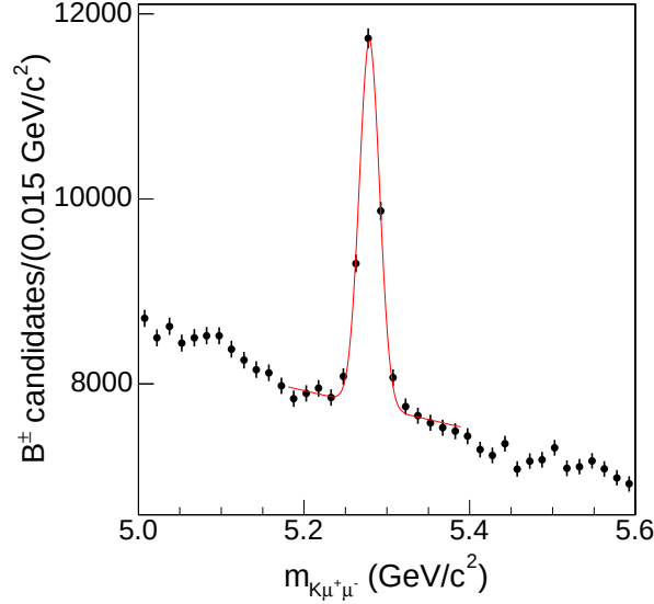
Figure 2: Invariant mass distribution of all B^\pm candidates. The line represents a fit to the data using a first order polynomial plus a gaussian function in order to estimate the background and the B^\pm signal, respectively.
