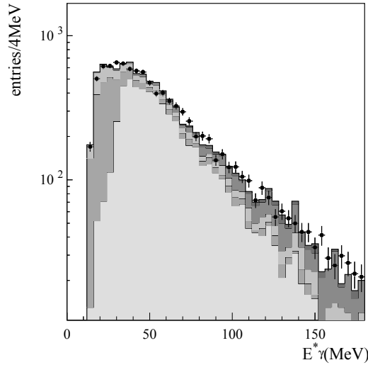
Figure 1: Photon energy spectrum observed in K_L \rightarrow \pi e \nu \gamma decays; data are represented by black points, MC shapes for signal (light gray) and background contribution added to signal (dark gray) are also reported.
