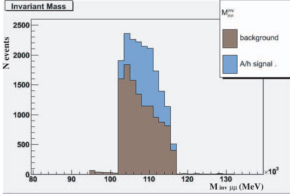
Figure 7: Distributions of the reconstructed \mu^+\mu^- invariant mass for signal and background events, after all selection cuts at the reference point ( \tan(\beta) = 45 , M_A = 110.31 GeV, M_h = 110.00 GeV). The two distributions are normalized at L = 300 \text{ fb}^{-1} . The h/A signal (light blue) emerges over background (Z, t-tbar and ZZ) (dark brown).
