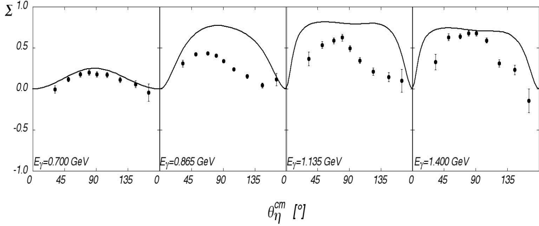
Figure 2: Preliminary result for beam asymmetry for \eta photoproduction from the neutron compared with MAID2001 prediction.
