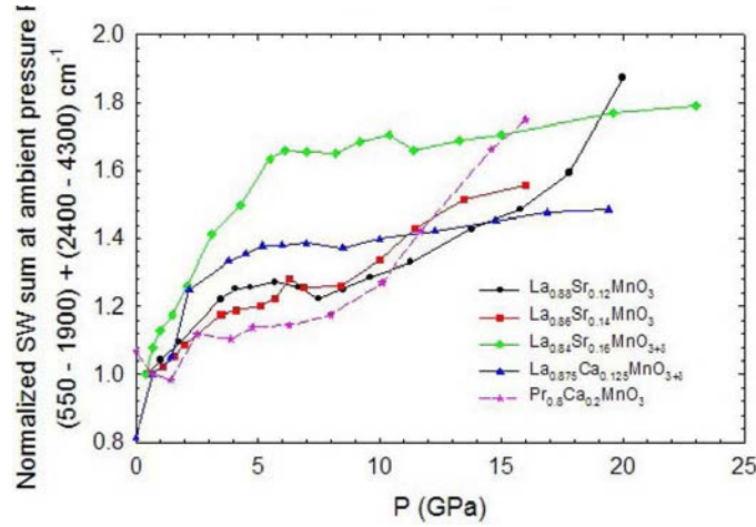
Figure 3: Sum of the low and high frequency spectral weight.
