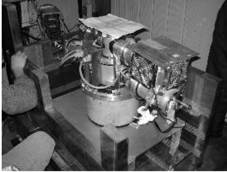
Figure 2: Installation of the VIP setup in Gran Sasso underground laboratory.
