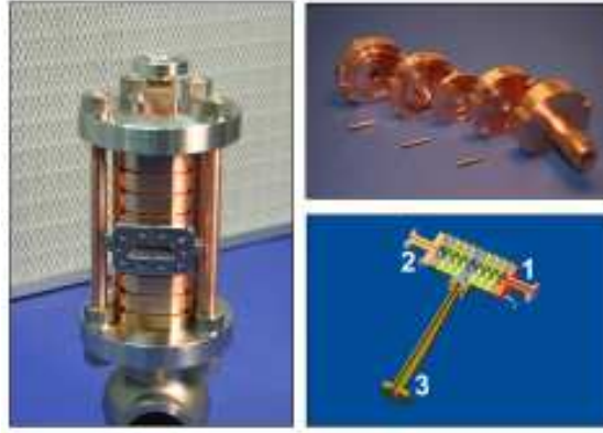
Figure 4: Copper prototype of the structure.
