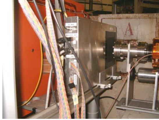
Figure 4: The silicon microstrip chamber before the the dipole
