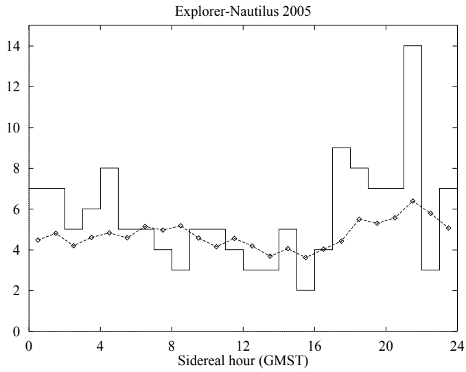
Figure 2: Explorer-Nautilus coincidences in 2005. Number of coincidence and average accidentals as a function of sidereal hour.
