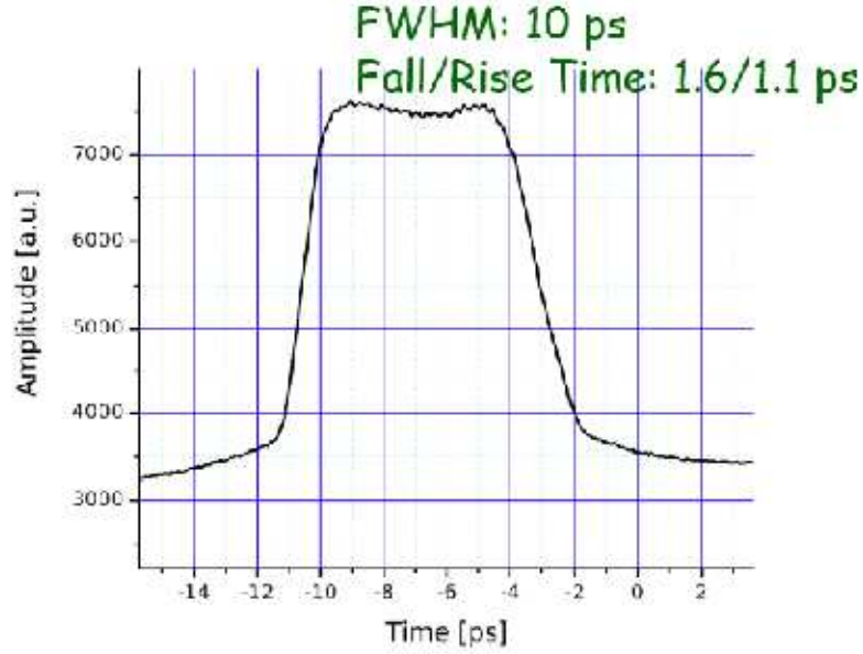
Figure 4: Measured flat top laser pulse, showing a 10 ps (FWHM) longitudinal profile with rise and fall time less than 2 ps.
