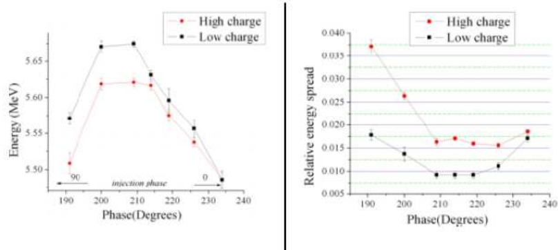
Figure 6: Energy (a) and energy spread (b) for low and high bunch charge.
