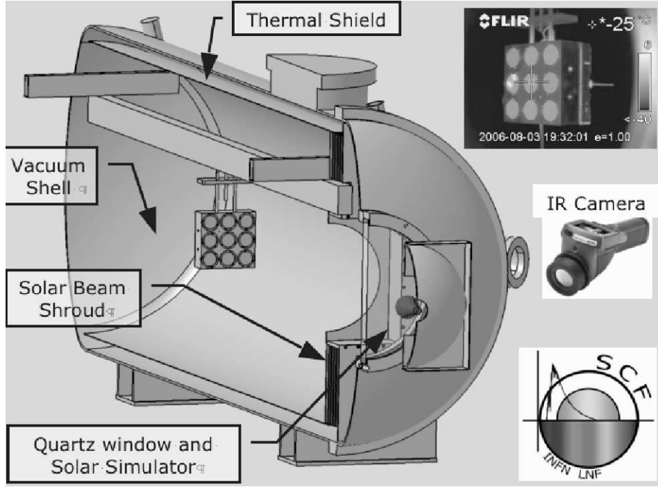
Figure 1: Sketch of the LNF Space Climatic Facility
