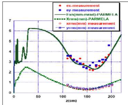
Figure 11: Envelope and emittance versus z for a Flat Top pulse.
