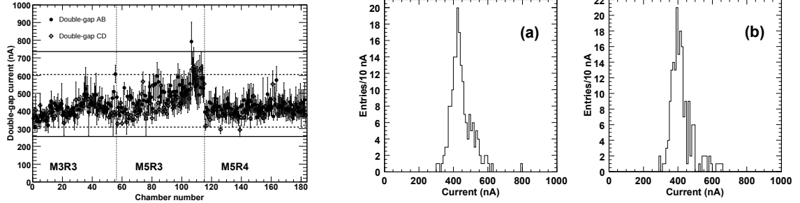
Figure 1: Average values of \langle I \rangle for the two double-gaps of the chambers produced in 2005, with the maximum spread found superimposed, after the correction for the T and P effects. (for the detailed explanation of the plots, you can refer to 3) and 4) )
