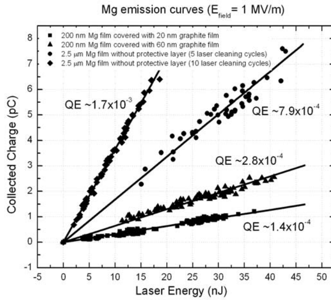
Figure 13: Emission curves of different Mg samples deposited by PLD on Cu substrates, after the laser cleaning of the protective or contaminated layers.
