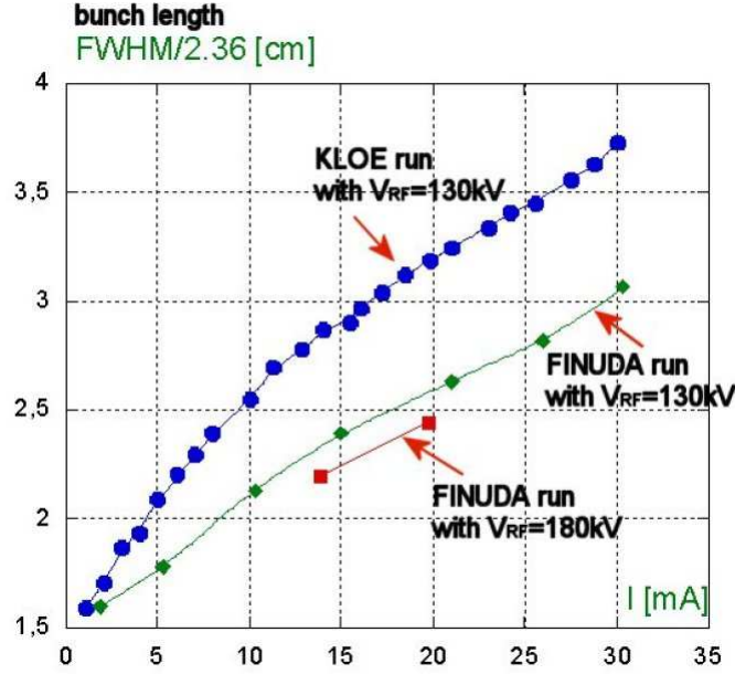
Figure 8: Bunch length measurement before and after the ICE removal.
