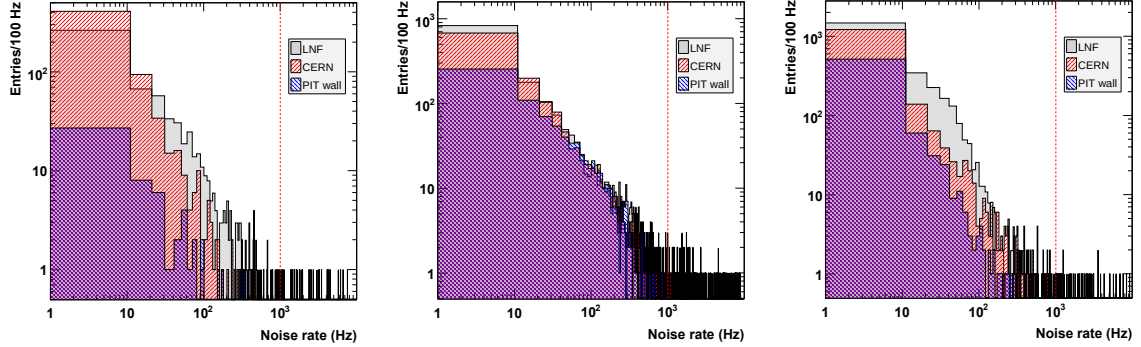
Figure 3: Noise values measured in LNF, CERN and PIT wall for M5R2 (left), M5R3 (center) and M5R4 (right) chambers.
