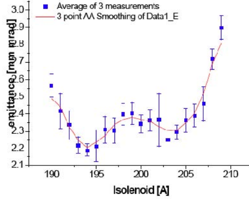
Figure 12: Emittance versus solenoid current at a fixed position , z=1.5 m.
