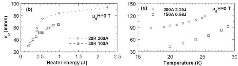
Figure 3: Normal zone propagation velocity as a function of both the heater energy (left) and the temperature (right)
