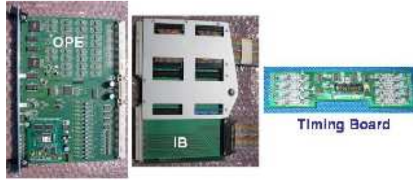
Figure 2: The picture shows the main elements of the timing system: the Timing Board, the Interconnection Board (IB), receiving the cables from 14 TBs, and the OPE Board, connected to the IB.
