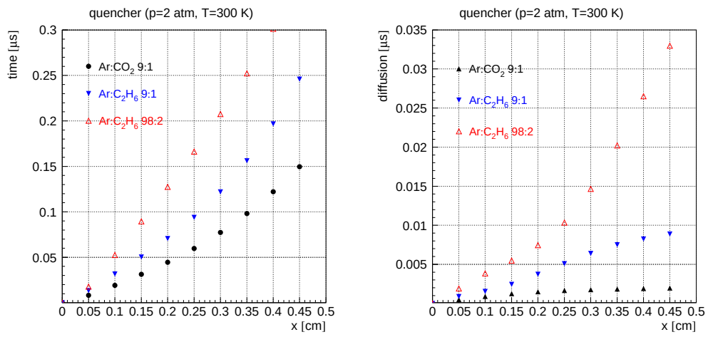
Figure 2: Behavior of different gas mixtures: (left) space time relation; (right) diffusion along the fastest drift path.
