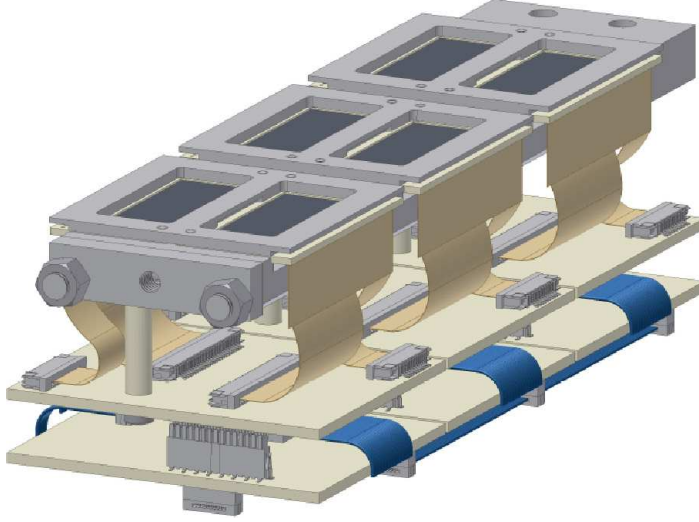
Figure 1: An 18 \text{ cm}^2 SDD unit, containing 18 SDD individual chips.
