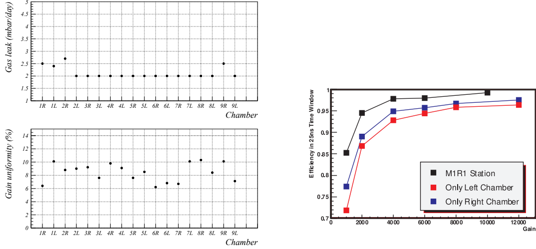
Figure 4: (a) Quality tests performed on the whole production: (top) Gas leak measured as loss of overpressure (mbar/day); (bottom) Gain uniformity. (b) Efficiency in the bunch crossing time window (25ns) as a function of detector gain, for the station (black) and with only one chamber switched on (red and blue). The FEE threshold was about 3fC
