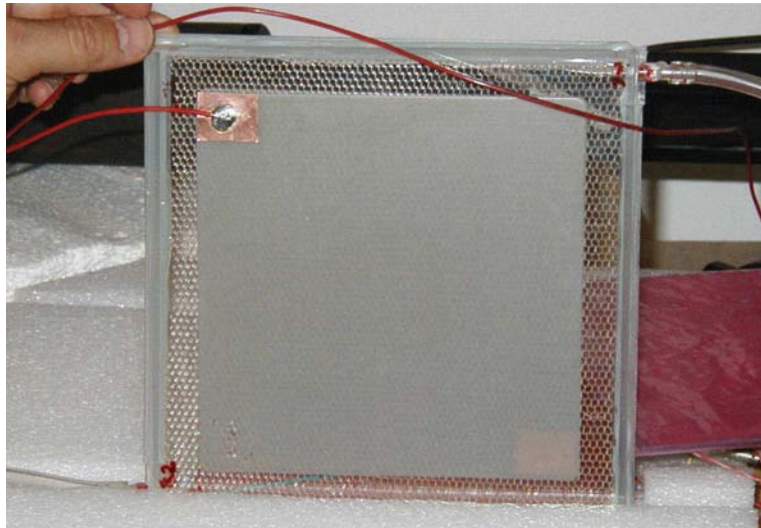
Figure 1: One of the mechanically quenched parallel plates detectors.
