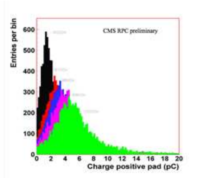
Figure 6: Charge distribution of single gap operated in avalanche regime and read by two 45cm x 45cm pads. The high voltage is increased from 9.5kV to 10kV. Pedestal is subtracted.
