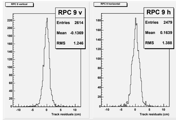
Figure 3: Examples of tracking residuals of one RPC layer, for the bending projection (plot at left) and for the non-bending projection (plot at right).
