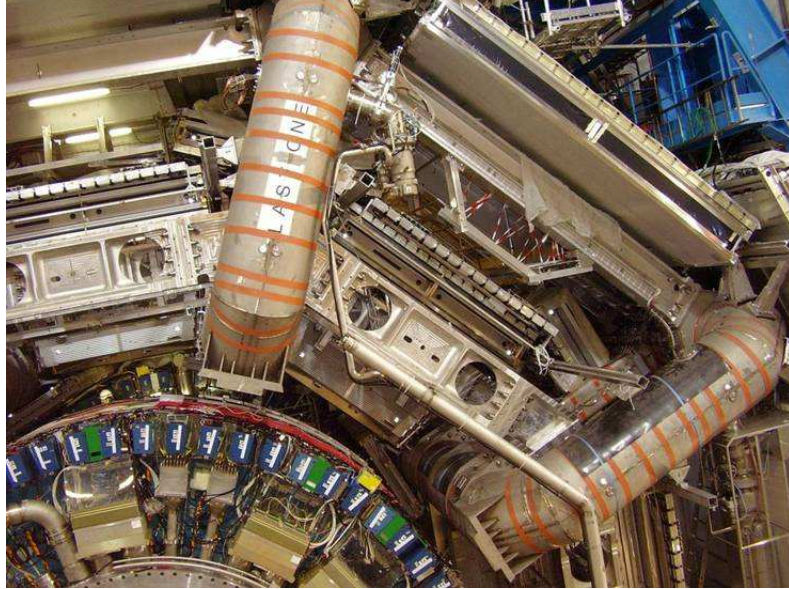
Figure 1: An enlarged view of the top region of the Muon spectrometer
