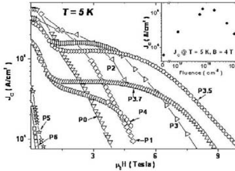
Figure 1: Critical currents measured in samples which had different neutron doses
