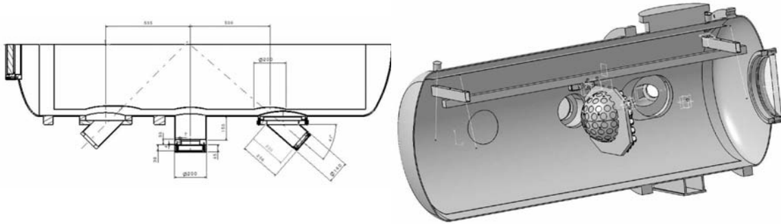
Figure 4: Upgraded SCF. Left: top view (Sun enters left). Right: side view (Sun enters right).
