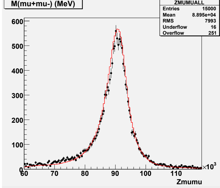
Figure 10: Invariant dimuon mass for the calibration sample of 15000 Z \rightarrow \mu^+\mu^- selected events: (black points) offline reconstructed mass, (solid line) mass reconstructed by folding the generated particle spectra with MC resolution.
