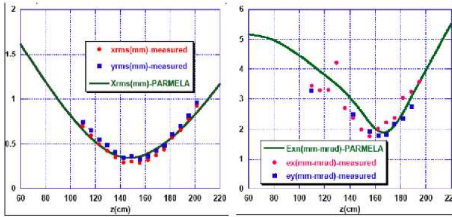
Figure 10: Envelope and emittance versus z for a Gaussian pulse.
