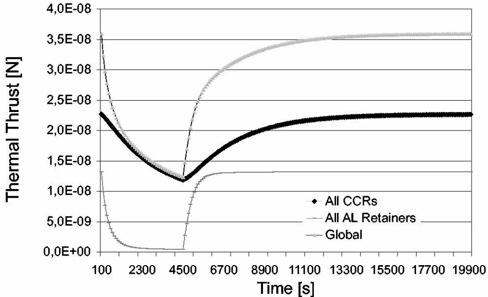
Figure 2: Parametric simulation of the thermal thrusts on LAGEOS due to the SCF Sun and Earth simulators for CCR solar absorptivity = 1.5%.
