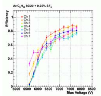
Figure 3: Plateaux curves for the six detectors built with Hexcell structure in the gas volumes. The curve number 7 refers to a “traditional” RPC.
