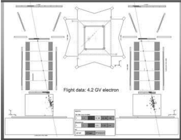
Figure 4: Display of an in-flight 4.2 GeV electron
