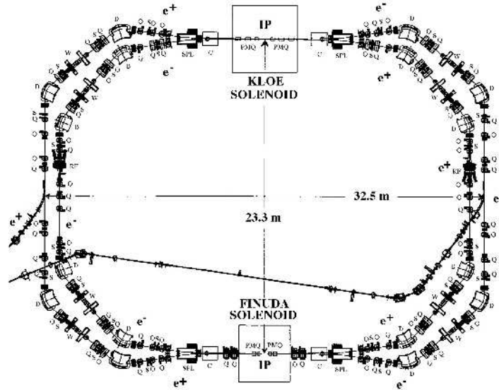
Figure 2: The DAΦNE Main Rings.
