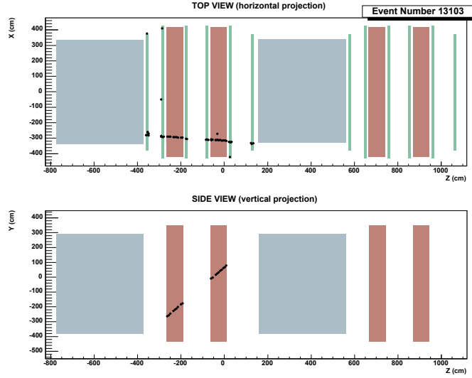
Figure 4: Event reconstructed in the drift tubes of the first spectrometer. Drift tubes are represented in green, while the iron magnet with the installed RPCs are plotted in brown. The other electronic detectors where off.
