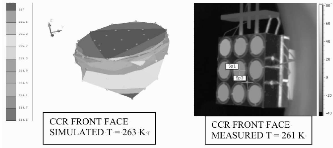
Figure 3: Simulated and measured temperature of the CCR in the SCF (Earth IR only).
