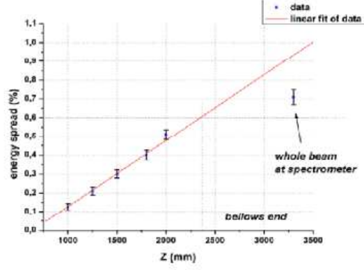
Figure 7: Energy spread versus z.
