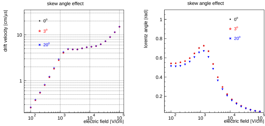
Figure 3: Effects of the skew angle on straw performance: (left) drift velocity; (right) Lorentz angle.
