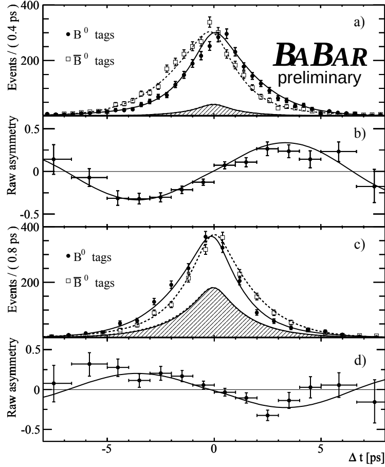
Figure 3: a) Number of \eta_f = -1 candidates ( J/\psi K_S^0 , \psi(2S)K_S^0 , \chi_{c1}K_S^0 , and \eta_c K_S^0 ) in the signal region with a B^0 tag ( N_{B^0} ) and with a \bar{B}^0 tag ( N_{\bar{B}^0} ), and b) the raw asymmetry (N_{B^0} - N_{\bar{B}^0})/(N_{B^0} + N_{\bar{B}^0}) , as functions of \Delta t . Figures c) and d) are the corresponding distributions for the \eta_f = +1 mode J/\psi K_L^0 . The solid (dashed) curves represent the fit projections in \Delta t for B^0 ( \bar{B}^0 ) tags. The shaded regions represent the estimated background contributions.
