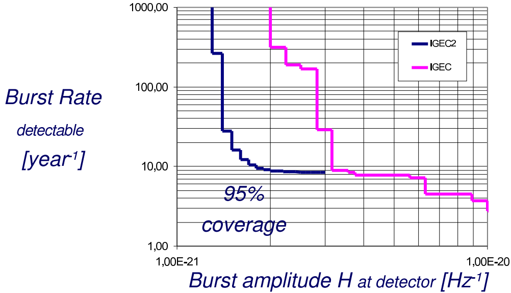
Figure 3: Upper limit at 95% on the rate of detectable GW events as a function of the threshold in amplitude used in the search.
