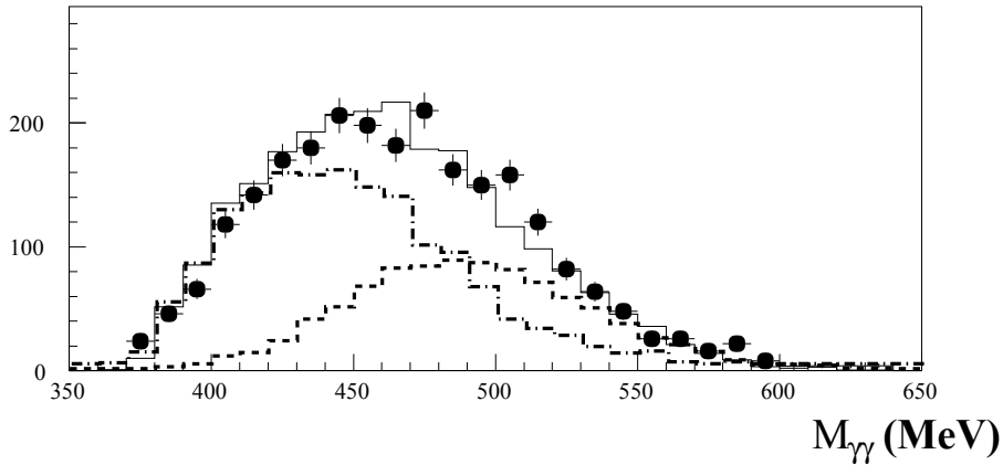
Figure 2: Two-photon invariant mass as observed at the end of K_S \rightarrow \gamma\gamma selection procedure; black points are data, dashed and dot-dashed lines signal and background components, respectively, obtained using MC-predicted shapes for both contributions.
