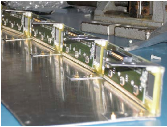
Figure 5: The tagging modules mounted on the new supporting structure
