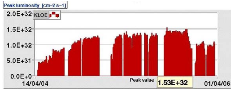
Figure 3: Evolution of the DAFNE peak luminosity since April 2004 (KLOE run).
