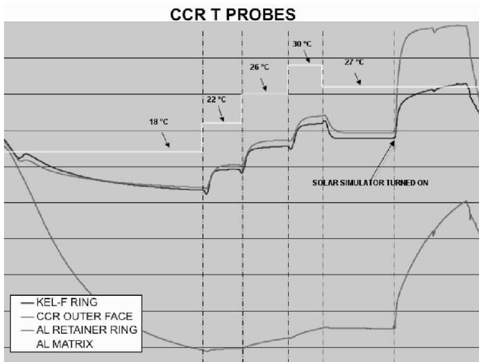
Figure 4: Space-climatic test of the LAGEOS 3x3 CCR matri prototype at the SCF with the Sun Simulator only. Temperature (AU) of CCR and its mounting rings vs. time (AU).
