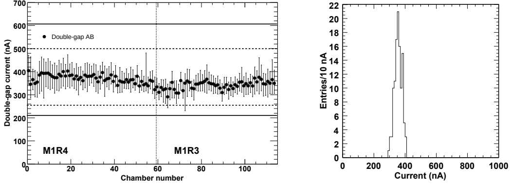
Figure 2: Average values of \langle I \rangle for the two double-gaps of the M1R4 chambers, with the maximum spread found superimposed, after the correction for the T and P effects. (for the detailed explanation of the plots, you can refer to 3) and 4) )
