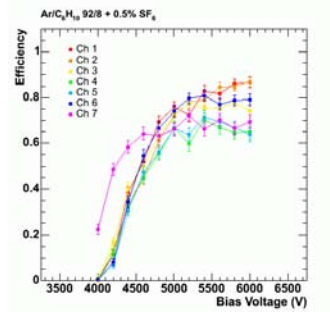
Figure 2: Plateaux curves for the six detectors built with Hexcell structure in the gas volumes. The curve number 7 refers to a “traditional” RPC.
