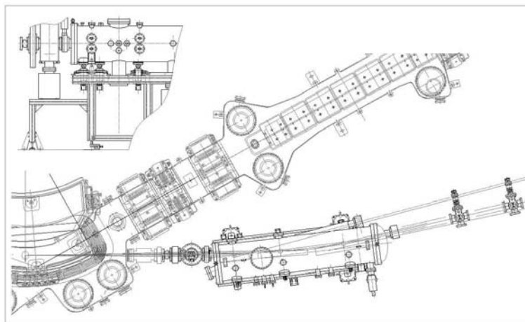
Figure 4: Constructive drawing of the optical UHV chamber and of the front end to be installed in the summer 2007 (courtesy of RMP).
