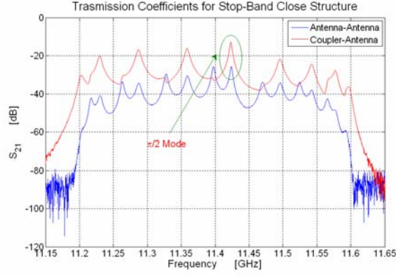
Figure 5: Transmission coefficient between the two lateral antenna in stop-band close case.
