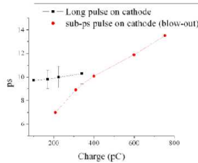
Figure 8: Bunch length measurements with streak camera.
