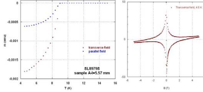
Figure 2: Magnetic moment for low filament size NbTi wire
