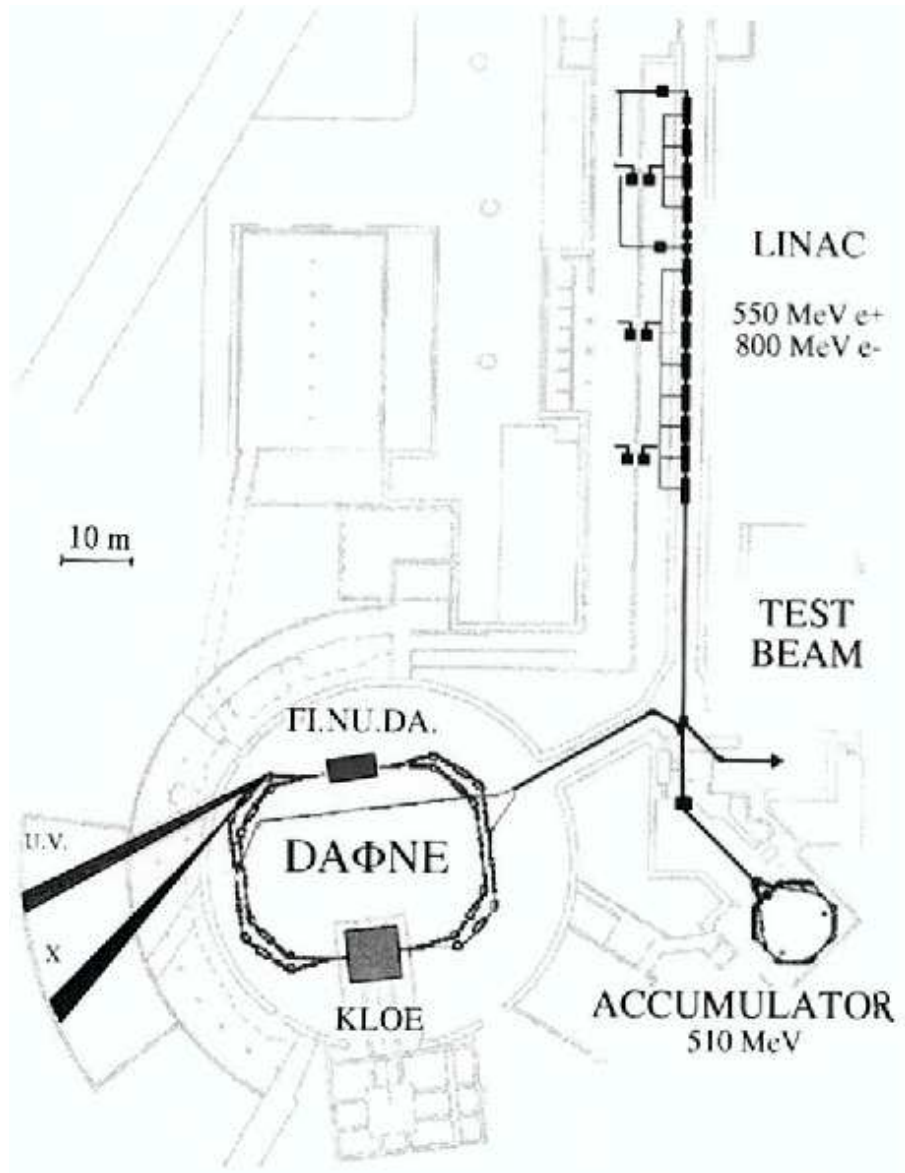
Figure 1: The layout of the DAΦNE accelerator complex inside its buildings.
