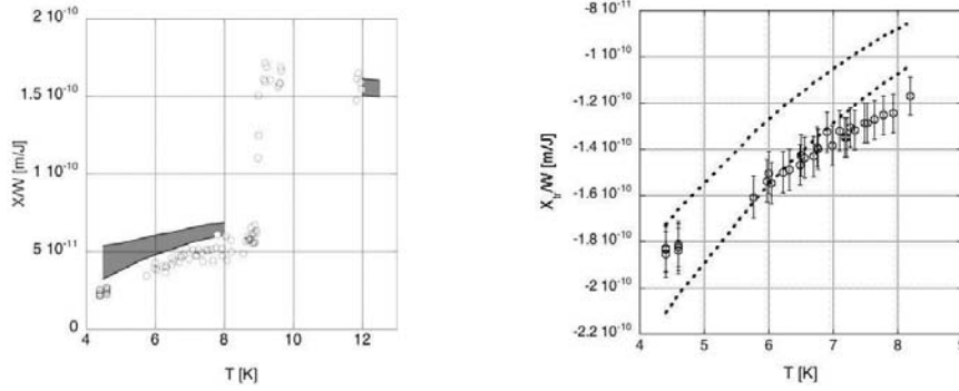
Figure 2: Nb - Left: FLMO maximum amplitudes ( X ) normalized to the total energy lost per beam pulse ( W ) vs. temperature ( T ). Circles: measured values. Bands: expected values. Right: The component of the FLMO maximum amplitude due to local transitions normalized to the energy lost ( X_{tr}/W ) vs. temperature ( T ). Circles: observed values. The region enclosed by the broken lines shows the expected values.
