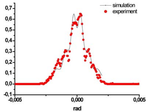
Figure 3: Image of ODR angular distribution (left) and its projection on the orizontal axis compared with the theoretical distribution from a beam with the measured parameters (right).
