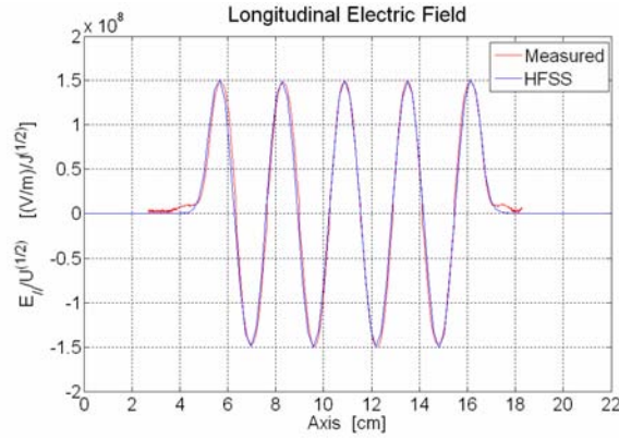
Figure 7: Measured longitudinal electric field on axis.
