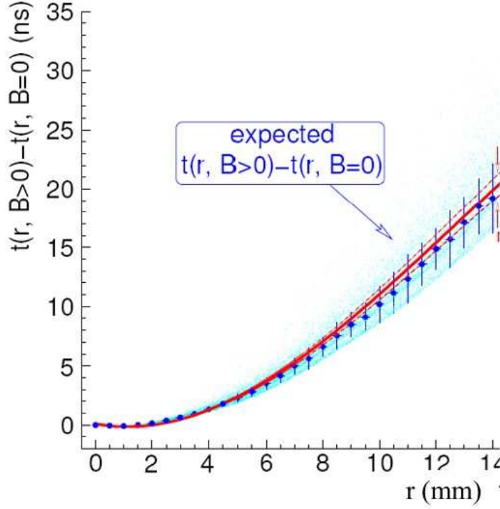
Figure 4: Effect of the magnetic field on MDT drift
