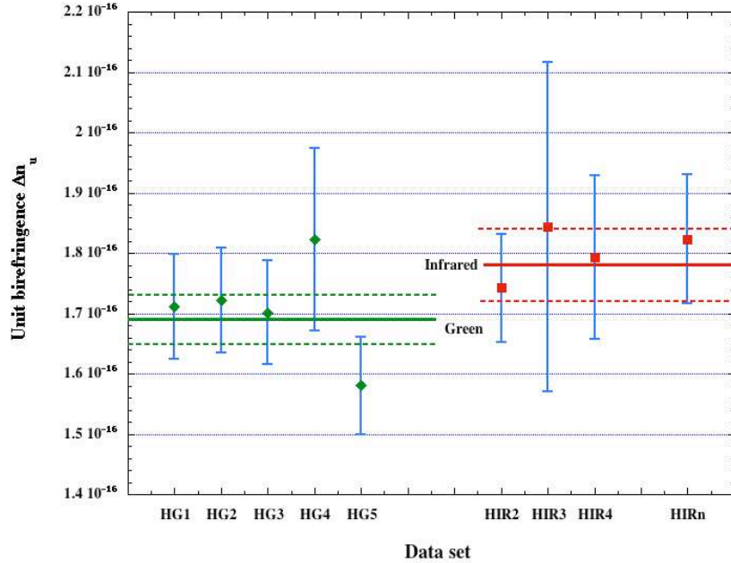
Figure 2: Unit birefringence of He as a function of data set. Green refers to a laser wavelength of 532 nm while Infrared refers to 1064 nm. Different data sets were acquired at different times spanning about two years from HG1 to HIRn. The dotted lines represent 1σ error bands. Notice the stability of the apparatus over time.
