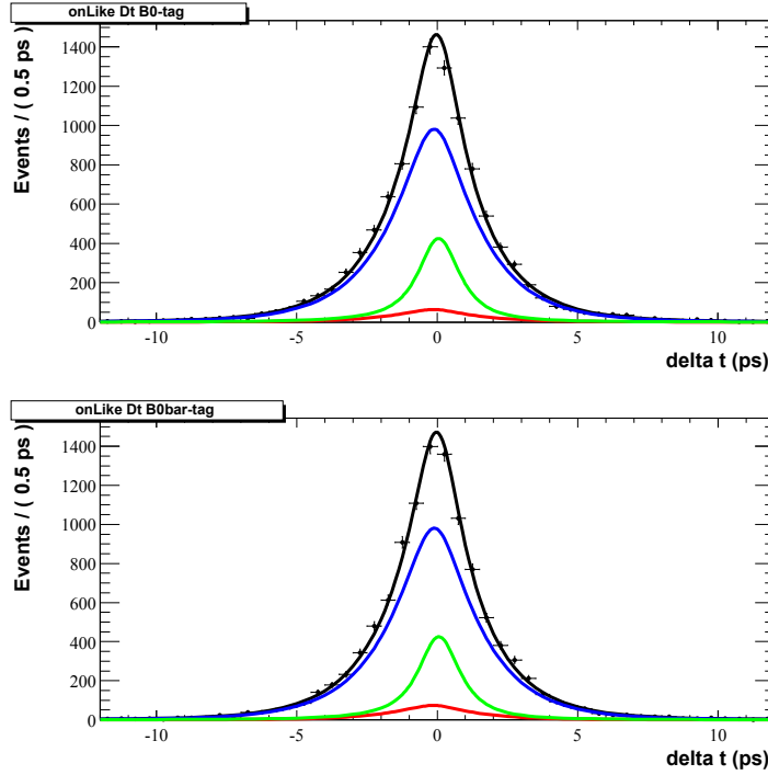
Figure 5: \Delta t fit to RUN 1-5 data. The curves represent the p.d.f.'s for signal (red), continuum background (green), B\bar{B} background (blue) and their sum (black).
