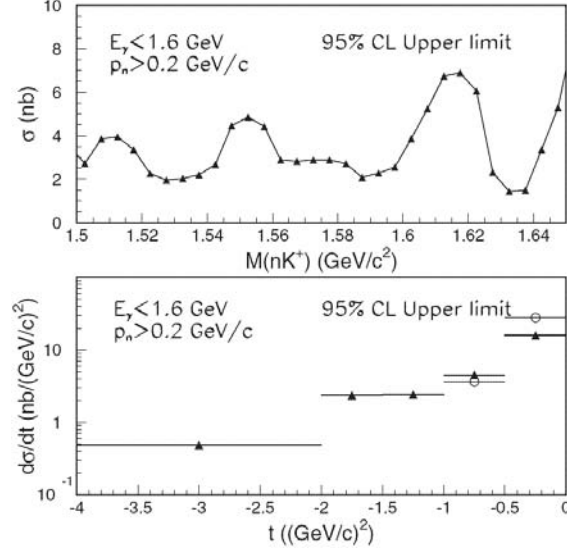
Figure 1: Top: 95% confidence level upper limit of the \gamma d \rightarrow \Lambda \Theta^+ reaction total cross section as a function of the nK^+ invariant mass. Bottom: 95% confidence level upper limit of the differential cross section d\sigma/dt as a function of t , for 1.52 < M(nK^+) < 1.56 \text{ GeV}/c^2 . The triangles and the circles represent the results obtained using two different model for the acceptance calculation.
