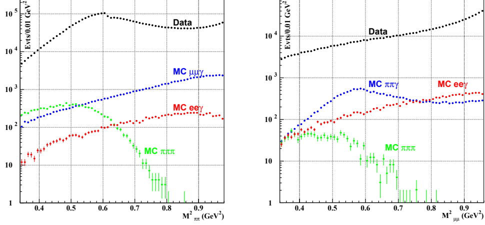
Figure 10: Number of \pi\pi\gamma(\gamma) (left) and \mu\mu\gamma(\gamma) events (right) obtained from 242 \text{ pb}^{-1} of data, with MC expectation for background contributions.
