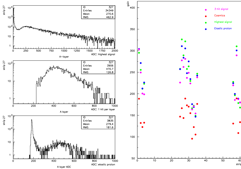
Figure 2: Left: Tree types of event selection for the Photon Detector, requiring everytime a lepton track in the forward spectrometer. On top the ADC spectrum in the case that strip A27 gave the highest signal in the Photon Detector A layer for this event; on the middle the ADC spectrum, of strip A27 in case of 1 hit in each of the three Photon Detector layers and on the bottom the signal of the elastic proton peak. Right: Comparison of the previous plot with cosmic test: the three cases are always higher than cosmics because of protons.
