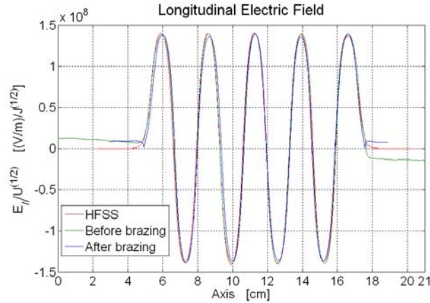
Figure 3: Measured longitudinal electric field on axis.
