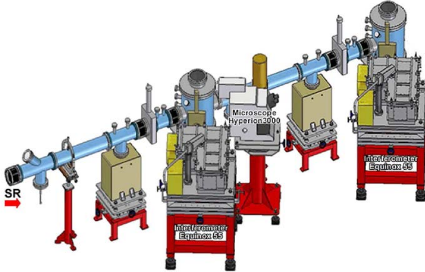
Figure 1: Layout of the two end stations installed on the SINBAD IR beamline.
