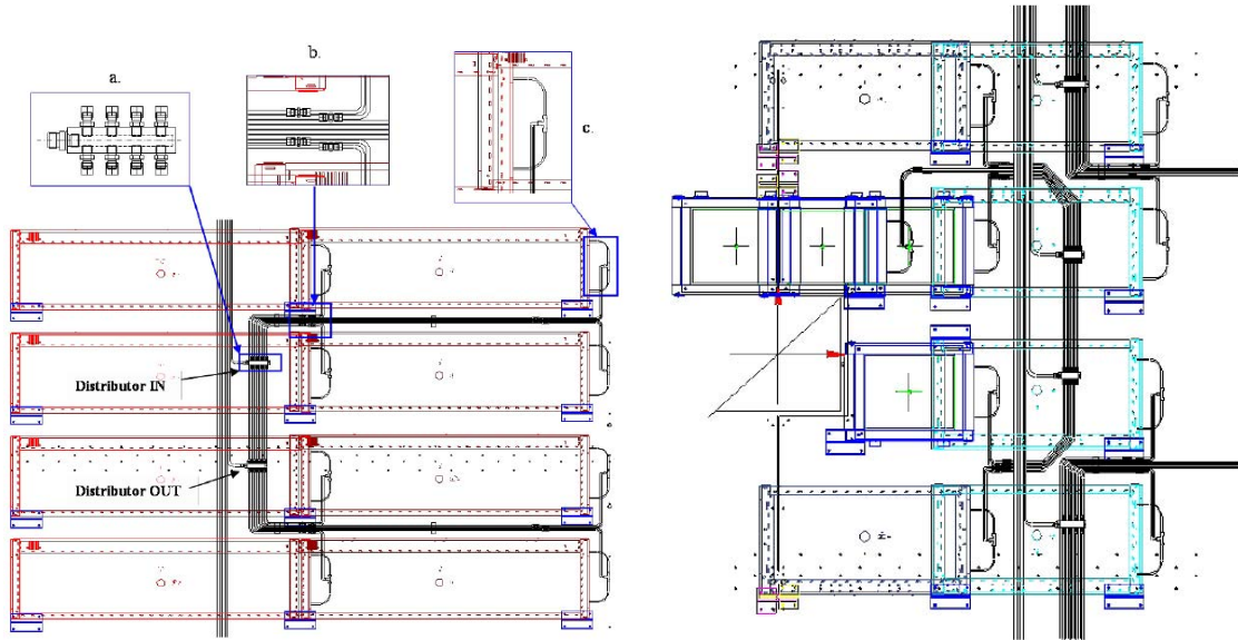
Figure 5: (a) Left: Design of Gas Line 1; a. Distributor IN; b. Connectors between copper and plastic tube; c. T connector with plastic tube. (b) Right: Design of Gas Line 9. This Gas Line supplies 5 chambers: 2 R2 and 3 R1.
