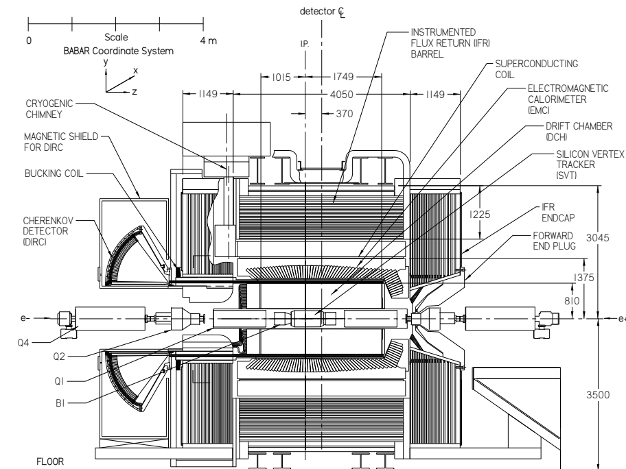
Figure 1: Elevation view of the BABAR Detector.
