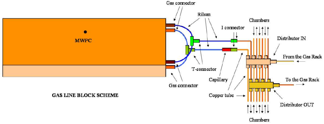
Figure 6: Scheme of a single gas line.
