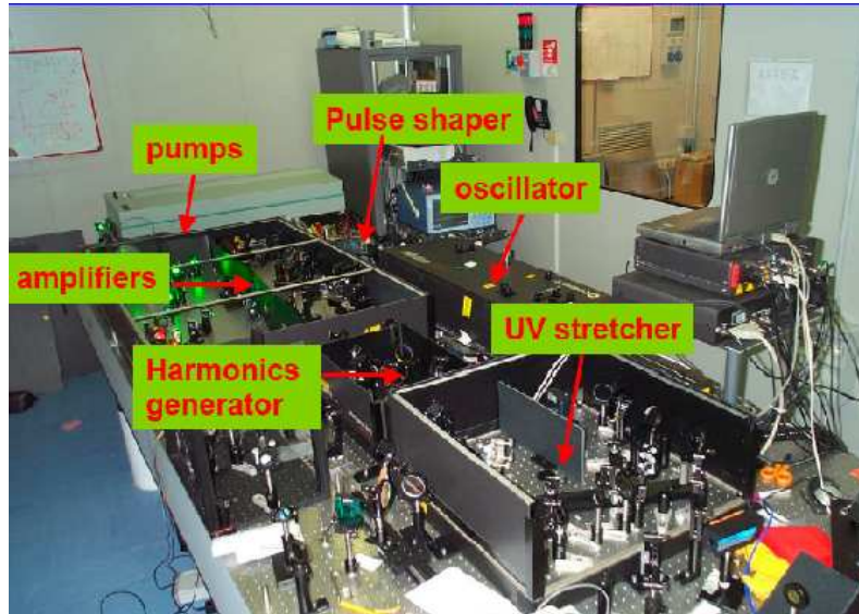
Figure 3: Laser system layout.
