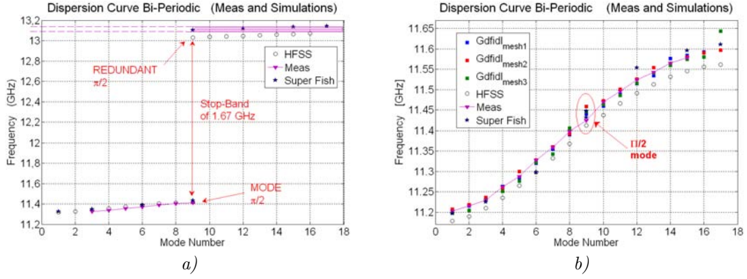
Figure 6: Measured dispersion curve in the case of: a) stop-band open and b) stop-band close, compared to simulation results.
