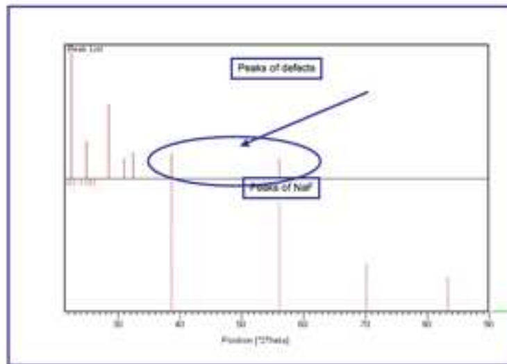
Figure 3: XRD spectrum of defects in a chamber irradiated at GIF. A very good match is observed for two characteristic peaks of NaF.
