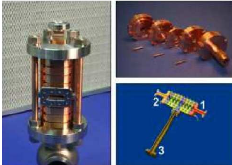
Figure 14: Copper prototype of the structure.
