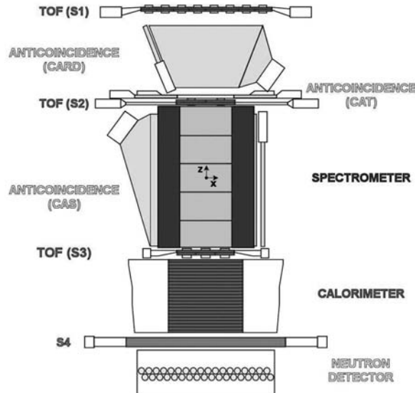
Figure 2: Sketch of the flight detectors the PAMELA telescope.
