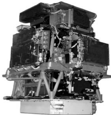
Figure 3: The PAMELA Flight Model.
