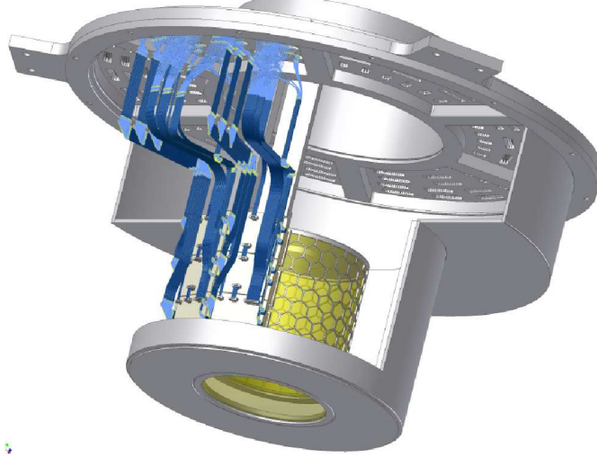
Figure 2: The SIDDHARTA target cell surrounded by SDD units (detail).
