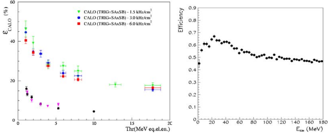
Figure 1: (Left-plot) Calorimeter detection efficiency (upper points) and expected efficiency for an equivalent thickness of NE-110 (lower points) to neutrons of 5-175 MeV as a function of the threshold. (Right plot) Detection efficiency as a function of neutron energy as estimated by FLUKA.
