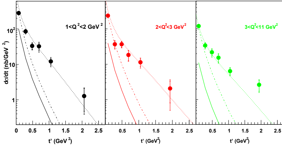
Figure 6: Cross section for exclusive \pi^+ production as function of t' for three different Q^2 ranges. The inner error bars represent the statistical uncertainty and the outer error bars the quadratic sum of statistical and systematic uncertainty. The curves represent calculations based on GPD and on Regge models.
