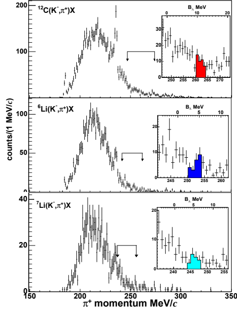
Figure 4: Inclusive \pi^+ momentum spectra of {}^6\text{Li} , {}^7\text{Li} and {}^{12}\text{C} targets. The insets show an enlarged view of the region where neutron rich \Lambda hypernuclei signals are expected.
