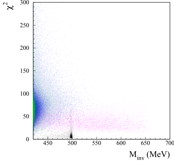
Figure 3: MC events as observed in M_{inv} - \chi^2 plane: points clustering at low \chi^2 values and M_{inv} = 500 \text{ MeV} are K_S \rightarrow e^+e^- events, while those at low M_{inv} values belong to K_S \rightarrow \pi^+\pi^-(\gamma) background, and those spread out over the entire M_{inv} window are \phi \rightarrow \pi^+\pi^-\pi^0 decays.
