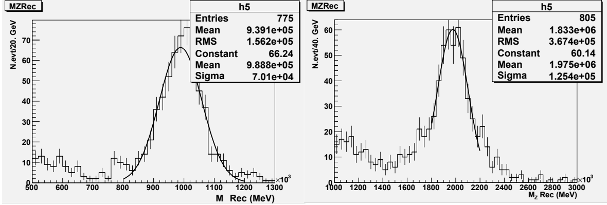
Figure 9: Distribution of dimuon invariant mass for pp \rightarrow \mu^+\mu^- events as expected by Drell-Yan, Z and Z' contributions for: (left) a Z' mass of 1 TeV and (right) of 2 TeV. The reconstruction is based on the Staco algorithm.
