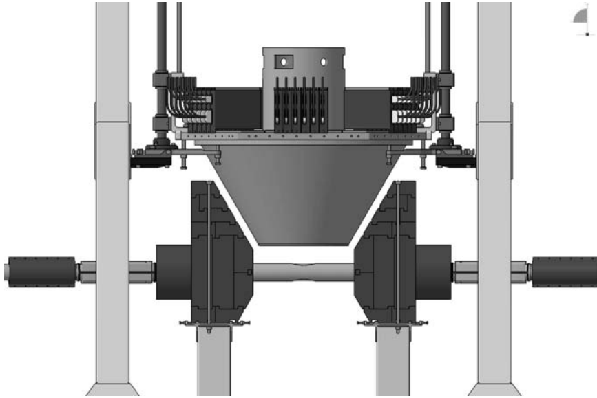
Figure 4: The schematic drawing of the SIDDHARTA setup in the Interaction Region of DAFNE.
