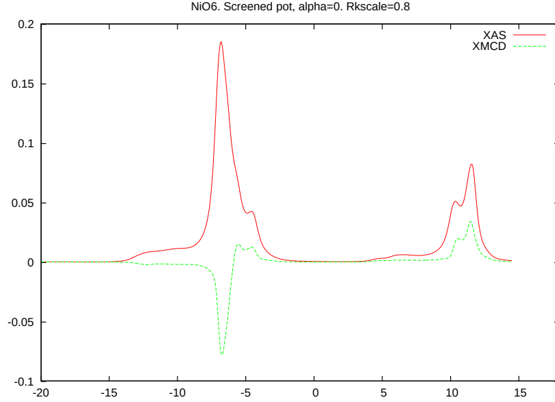
Figure 1: Calculated NiO L_3 L_2 Absorption edges. The branching ratio is back to its statistical value due to the Pauli principle. Also shown is the corresponding magnetic circular dichroism.
