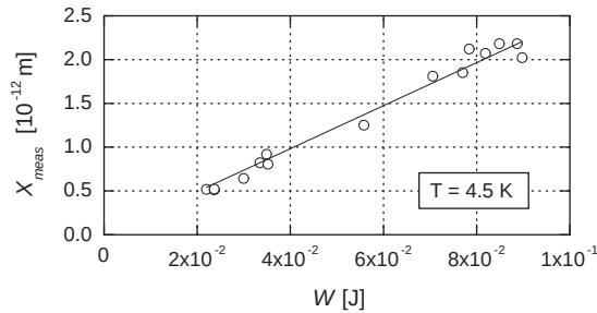
Figure 1: Nb, T = 4.5 K. Correlation between measured FLMO maximum amplitudes ( X_{meas} ) and energy ( W ), deposited by beam pulses in the bar, as derived by N_e measurements.
