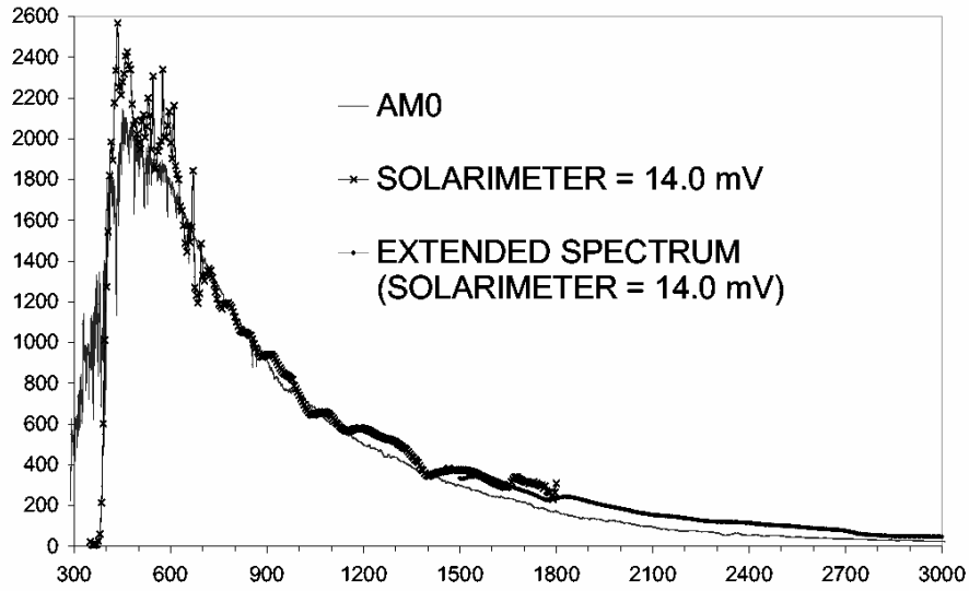
Fig. 3. The measured extended solar simulator spectrum ( \text{W}/\text{m}^2/\text{nm} \times 10^3 ) for \lambda > 1500 nm.
