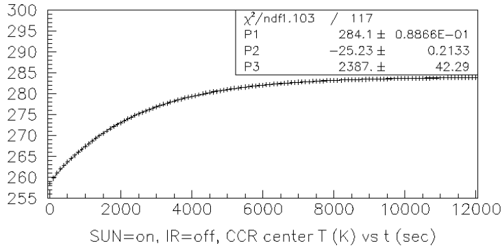
Fig. 5. LAGEOS matrix. Exponential fit to T(\text{CCR}) vs time in the simulation when the Sun is turned on at t > 0 , \alpha_{SUN} = 15\% and T(\text{AL}) = 300 K. P3 = \tau_{CCR} in seconds. This data assume a temperature accuracy of 0.5 K.
