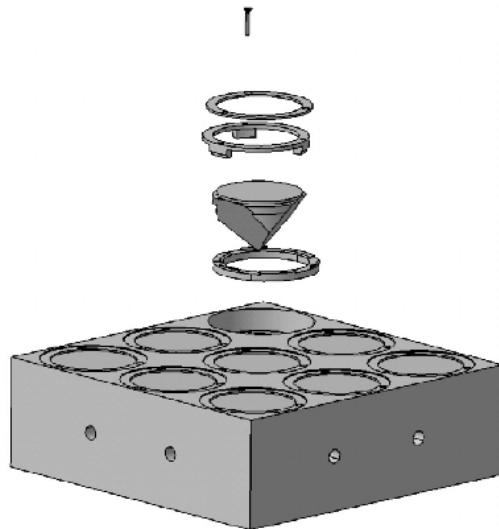
Fig. 4. The LAGEOS CCR assembly. The assembly elements facing outside (and, therefore, causing thermal thrusts) are the CCRs and the Al retainer rings (screws can be neglected).
