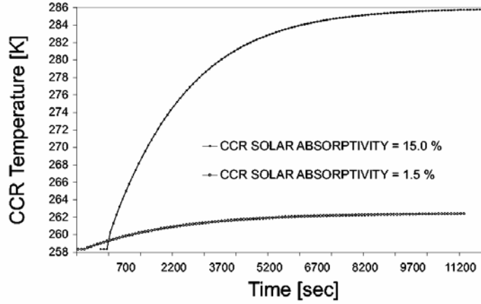
Fig. 7. LAGEOS matrix. Warm-up time of the CCR for \alpha_{SUN} = 15\% (top) and 1.5\% (bottom).
