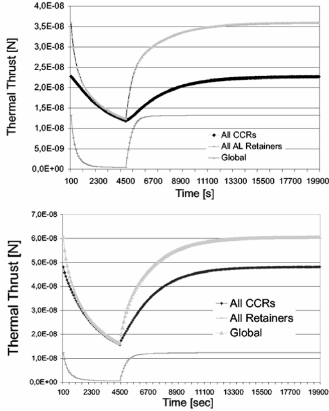
Fig. 9. LAGEOS parametric model. Estimate of the thermal thrusts on the satellite due to the SCF Sun and Earth simulators for \alpha_{SUN} = 1.5\% (top plot) and \alpha_{SUN} = 15\% (bottom plot).
