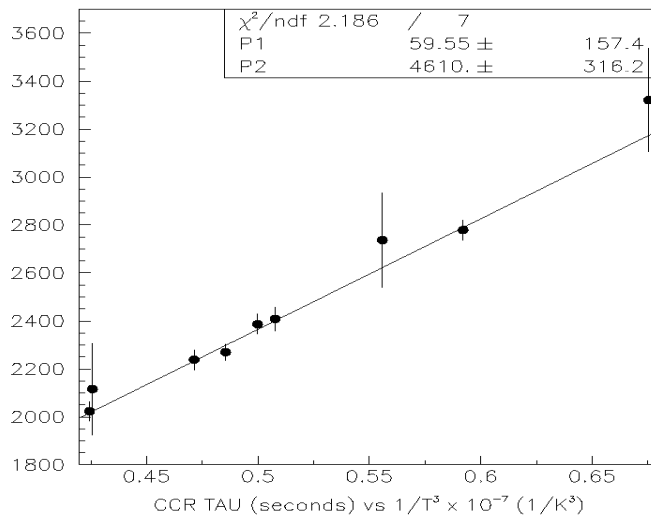
Fig. 6. LAGEOS matrix. \tau_{CCR} vs 1/T_{avg}^3 \times 10^{-7} in the simulation for \alpha_{SUN} = 15\% . Each point is a different set of conditions in terms of the Sun and Earth radiations, angle of exposure and value of T(\text{AL}) . For example, the first point is for T(\text{AL}) = 320 K, Sun = on, IR = off; the last point is for T(\text{AL}) = 280 K, Sun = on, IR = on. All other points are for T(\text{AL}) = 300 K.
