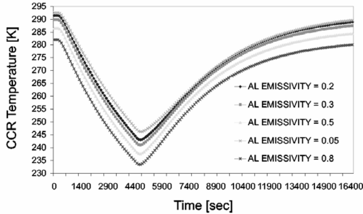
Fig. 8. LAGEOS matrix. Effect of Al ageing on T(\text{CCR}) for \alpha_{SUN} = 15\% . Sun off between 200 and 4700 sec (Earth shadow). The higher the value of \epsilon(\text{AL}) , the lower the T(\text{CCR}) curve.
