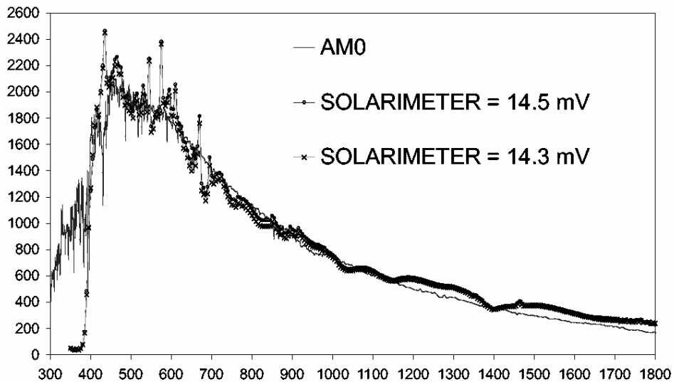
Fig. 2. AM0 spectrum ( \text{W}/\text{m}^2/\text{nm} \times 10^3 ) as a function of wavelength (nm) and two (almost undistinguishable) spectra measured with the SCF simulator, for two different values of the lamp currents and solarimeter readings. Typical currents are around 36 A (tungsten) and 29 A (HMI).
