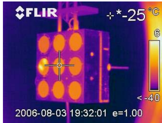
Fig. 11. Thermogram of the LAGEOS matrix taken with the IR camera through the Ge window.
