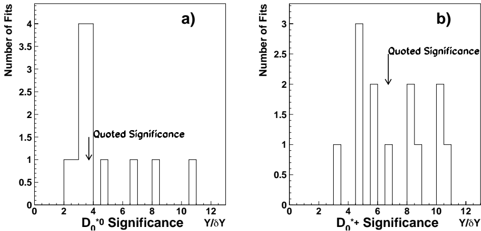
Figure 4: Statistical significance of broad states signals in the D^+\pi^- (a) and D^0\pi^+ (b) channels for various fits. The arrow indicates the significance of the result quoted.
