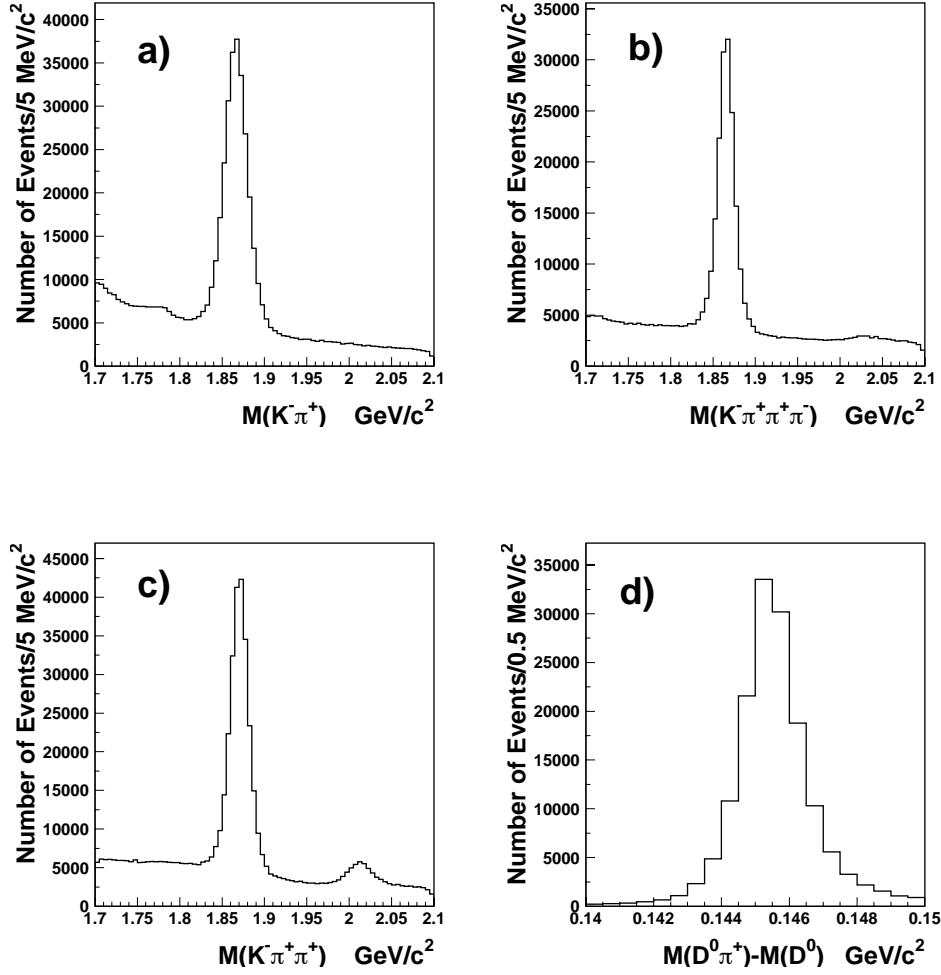
Figure 1: Invariant mass plots for: a) D^0 \rightarrow K^- \pi^+ ; b) D^0 \rightarrow K^- \pi^+ \pi^+ \pi^- ; c) D^+ \rightarrow K^- \pi^+ \pi^+ . Invariant mass difference plot for d) D^{*+} \rightarrow D^0 \pi^+ .
