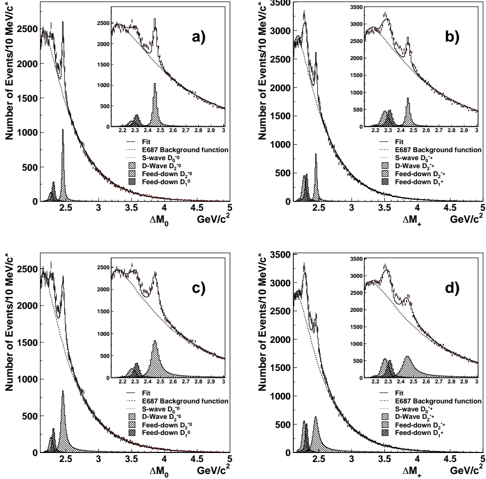
Figure 2: The fit to the D^+\pi^- and D^0\pi^+ mass spectra for the case where the D-wave mass and width are fixed to the PDG values, the background is described by Equation 3, and no broad resonance is included, is shown in a) and b). The case where the D-wave mass and width are allowed to float in the fit is shown in c) and d). Note that the none of these fits provides a good description of the data between the feed-downs ( \sim 2300 \text{ MeV}/c^2 ) and the D_2^* peak ( \sim 2500 \text{ MeV}/c^2 ). In Figure 3, we show that the data are well described when a broad resonance is included in the fit.
