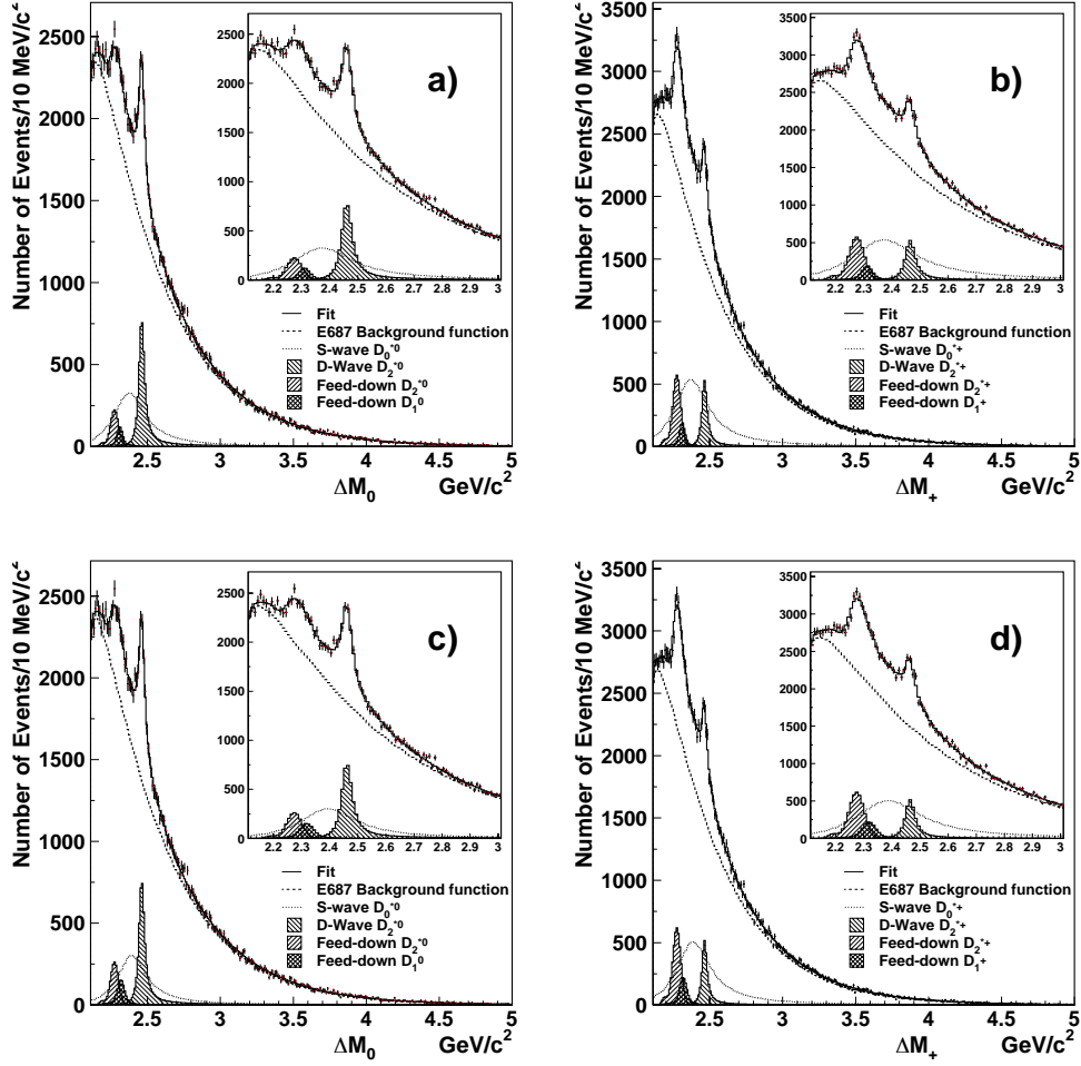
Figure 3: The fit to the D^+\pi^- and D^0\pi^+ mass spectra including a term for an S-wave resonance. The case with the mass and width for the D_1(3/2) and D_2^* feed-downs fixed to the PDG values is shown in a) and b). The case with the mass and width for the D_1(3/2) feed-down fixed to the PDG values and for the D_2^* feed-down determined by fits in a) and b) is shown in c) and d). Notice the excellent agreement when the broad resonance is included (described in more detail in the text).
