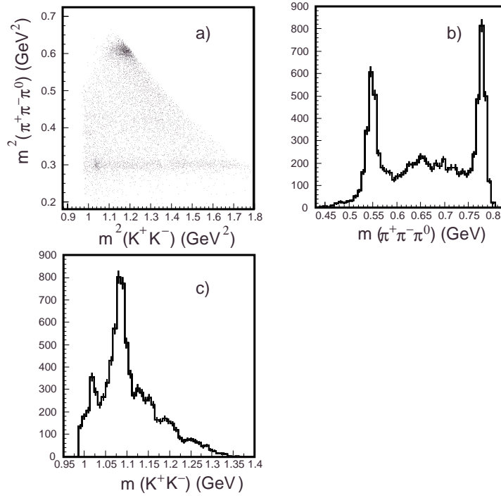
Figure 1: a) Scatter plot of m^2(\pi^+\pi^-\pi^0) versus m^2(K^+K^-) ; b) \pi^+\pi^-\pi^0 invariant mass; c) K^+K^- invariant mass.
