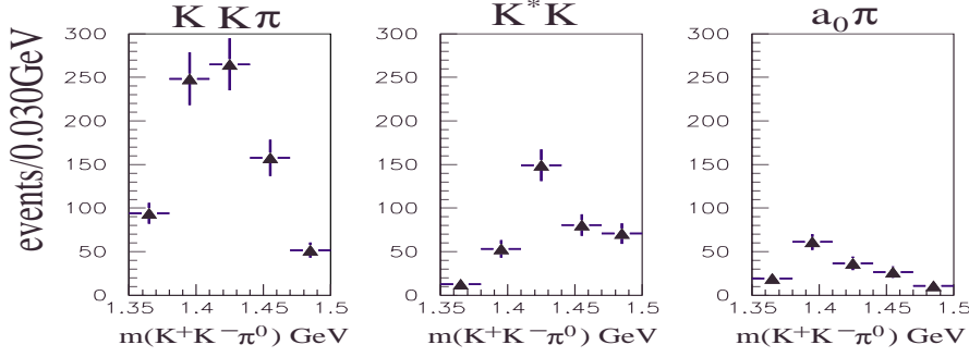
Figure 5: K^+K^-\pi^0 intensity spectra from the partial wave analysis of ^1S_0 initial protonium wave.
