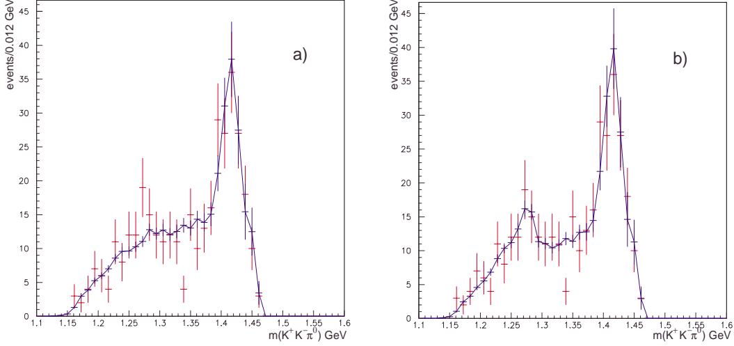
Figure 7: K^+K^-\pi^0 invariant mass spectrum with selection criteria applied to m(K^+K^-) and m(\pi^+\pi^-) , as described in the text. The lines superimposed to the experimental points are best fit solutions without (a) and with (b) the f_1(1285) in the amplitude.
