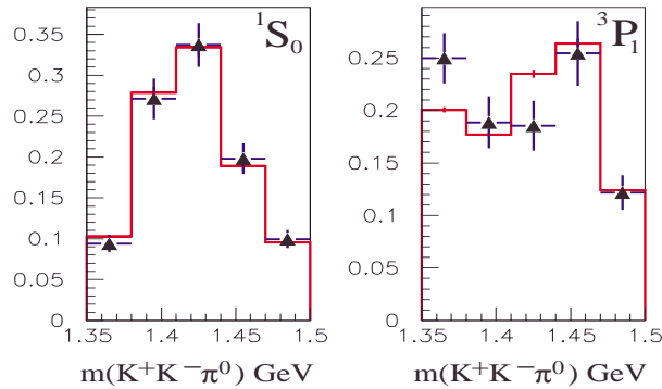
Figure 6: Comparison between the ^1S_0 and ^3P_1 partial wave intensities and the global fit results. The distributions are arbitrarily normalized to unity.
