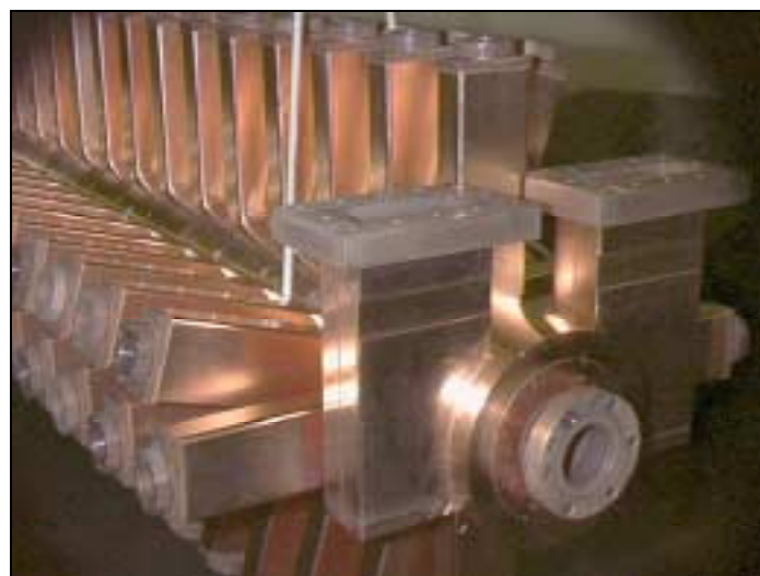
Figure 9.3 Brazen TDS ready for power testing
