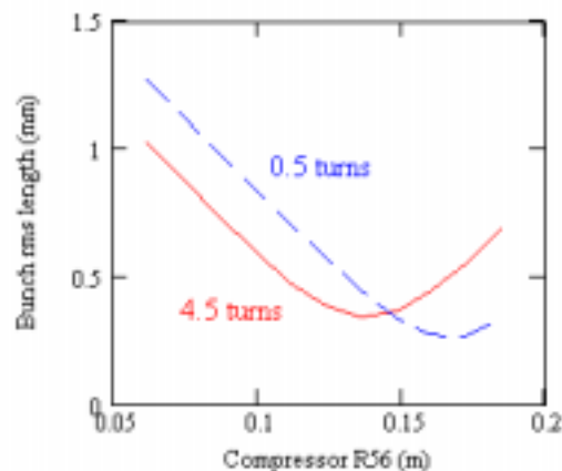
Figure 13.17 Bunch length as a function of the momentum compaction factor R_{56} in the final bunch compression system, for bunches making a different number of turns in the Combiner Ring.
