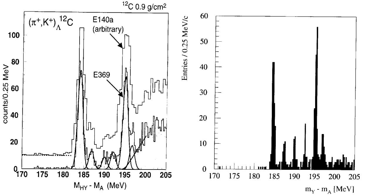
Figure 2: Left (from ref. [6]): hypernuclear mass spectrum of {}_{\Lambda}^{12}\text{C} from KEK experiments E369 and previous E140a with energy resolution of 1.45 MeV and 1.9 MeV (FWHM) respectively. Right : FINUDA simulation of the E369 {}_{\Lambda}^{12}\text{C} levels reconstructed with an energy resolution of 700 KeV (FWHM).
