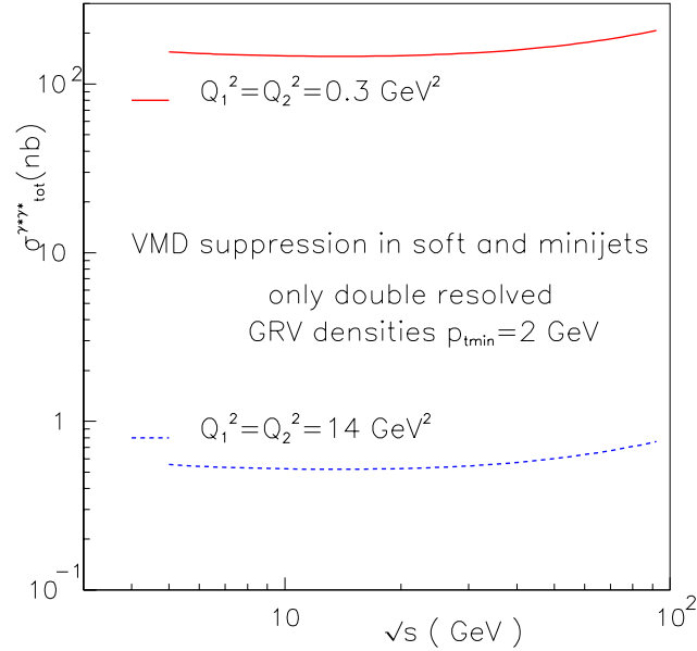
Figure 4: The EMM predictions for energy dependence of the double resolved part of virtual photons cross-section. Q_i^2 corresponds to the virtual photon mass
