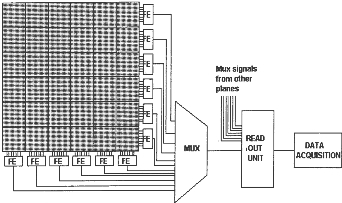
Fig. 4 General scheme of a detector plane and read out chain.
