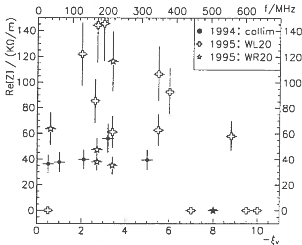
Figure 2: HERA-p effective transverse impedance as a function of chromaticity (frequency), computed from measured growth times
