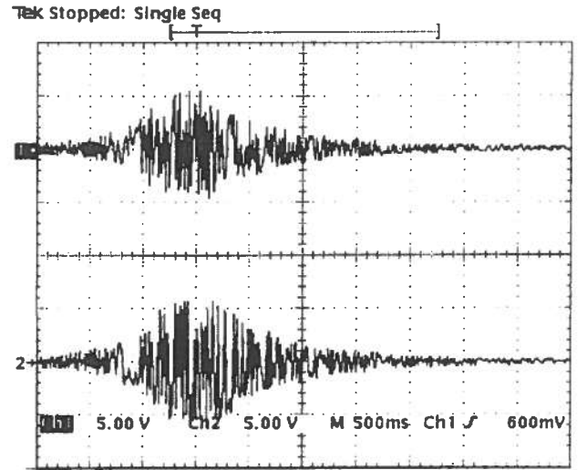
Figure 1: Growth time acquisition: the transverse position of the bunch center of charge as signal from horizontal and vertical pick-ups is displayed as a function of time
