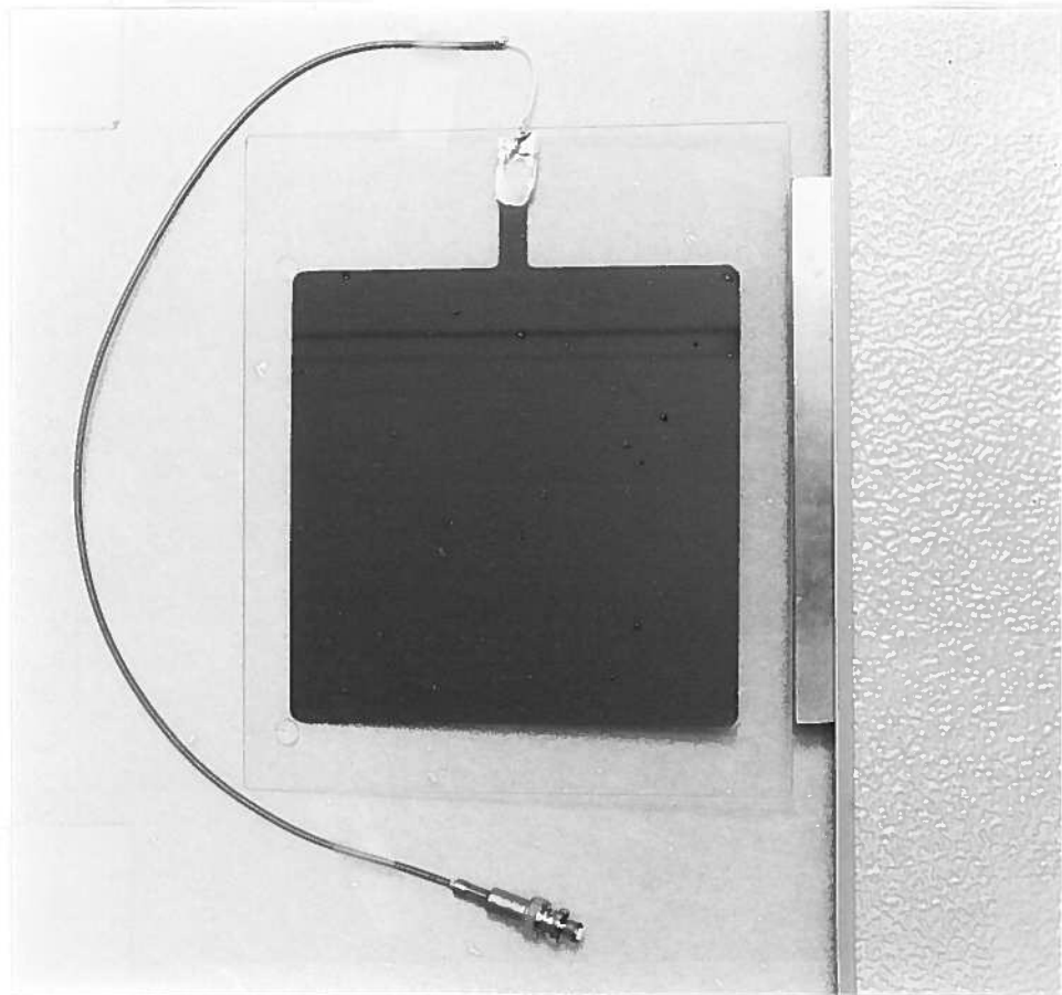
Fig. 3 - The resistive anode obtained using a germanium deposit on a glass plate.
