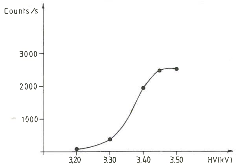
Fig. 9 - The dependence of the counting rate on the operating voltage when the chamber is irradiated with a ^{90}\text{Sr} source.
