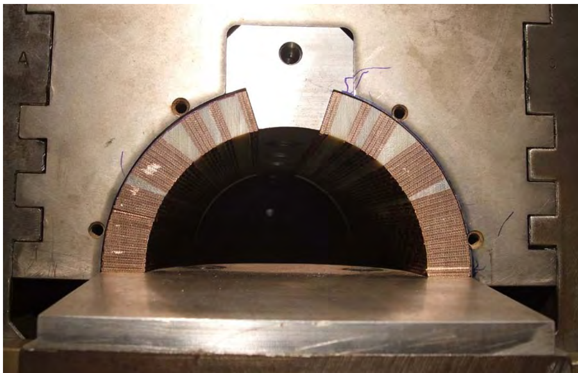
FIG.123: Arc piled sample for stress-strain measurements.
