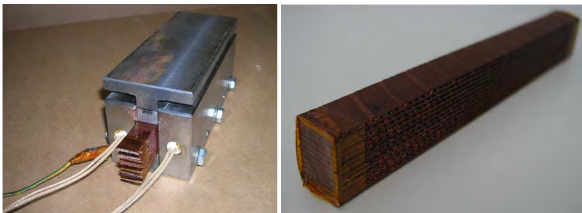
FIG.120: Stacked conductor ready to be cured, on the left, and a cured sample, on the right.
