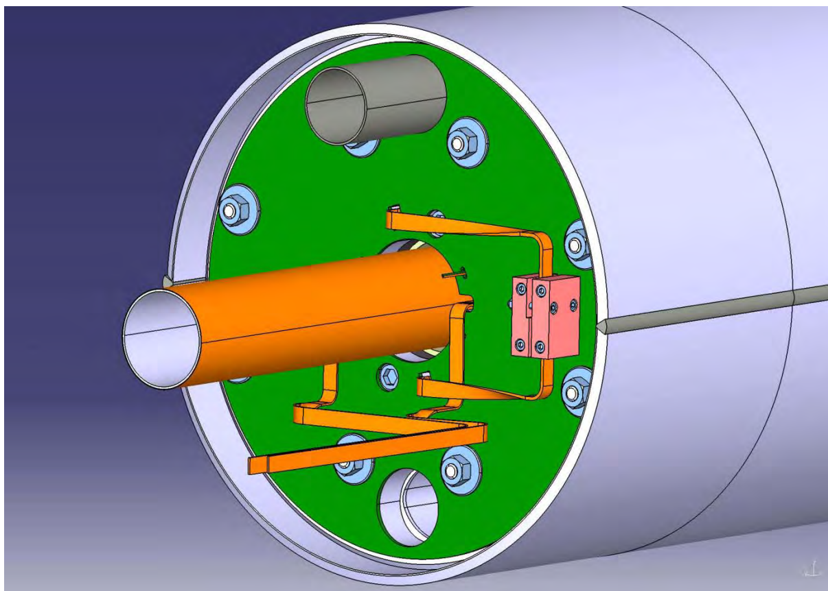
FIG.112: Conceptual scheme of the electrical exits.
