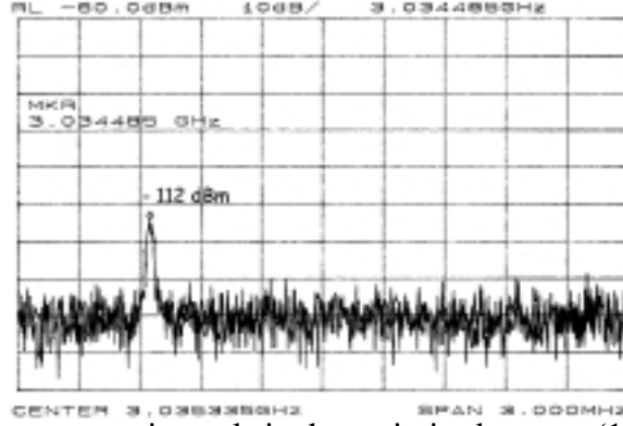
FIG. 4: Transmission of the symmetric mode in the optimised system (1 kHz resolution bandwidth; piezo off).
