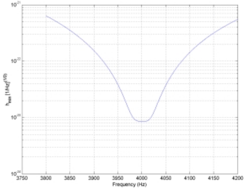
FIG. 8: Calculated system sensitivity for \omega_m = \omega_a - \omega_s = 4 kHz.
