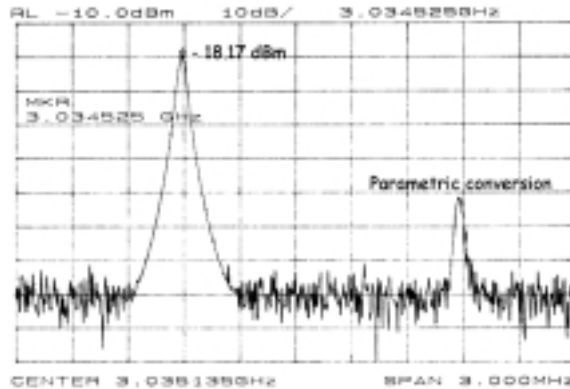
FIG. 3: Transmission of the symmetric mode (no optimisation) measured at the \Delta port of the output magic-tee (left peak) and antisymmetric mode excited by the piezo (right peak).
