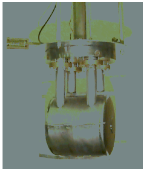
FIG. 1: PACO cavity mounted on the test cryostat.
