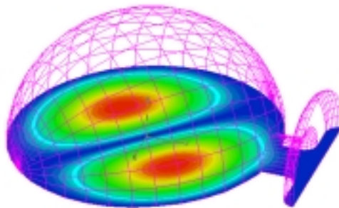
FIG. 9: Electric field magnitude of the TE011 mode. Note the alignment of the field axis.
