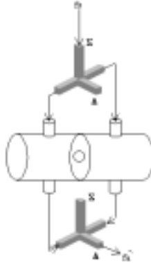
FIG. 2: Schematic view of the transmission detection scheme with two magic-tees.
