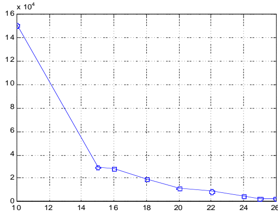
FIG. 6: Tuning sensitivity vs. cell half-distance.
