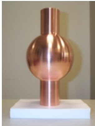
FIG. 10: Single cell, seamless, spherical cavity, built at INFN-LNL, to be sputter coated at CERN.
