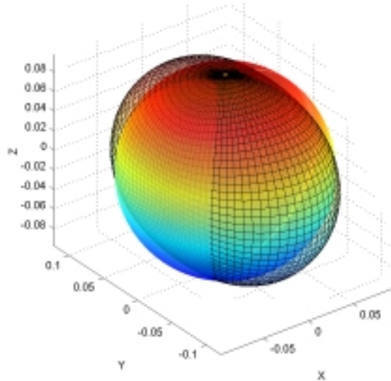
FIG. 7: Calculated deformation of an hollow sphere when the fundamental quadrupolar mechanical mode is excited.
