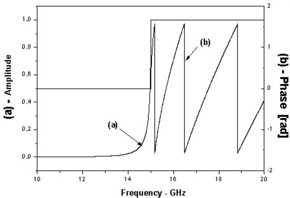
Fig. 12 – The transfer function corresponding to the new setup in Fig. 10. Its magnitude and phase are represented by lines (a) and (b), respectively.
