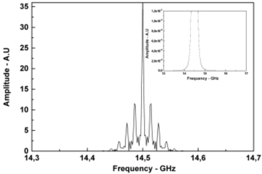
Fig. 14 – Spectrum of the entering signal. In the inset, the vertical scale was magnified 3 \times 10^4 times.
