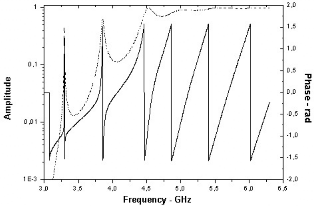
Fig. 7 – The transfer function corresponding to the setup in Fig. 6. Its magnitude and phase are represented by the pointed and solid lines, respectively. Notice that the intervals in which the phase derivative is lower coincide with the dips of the magnitude.
