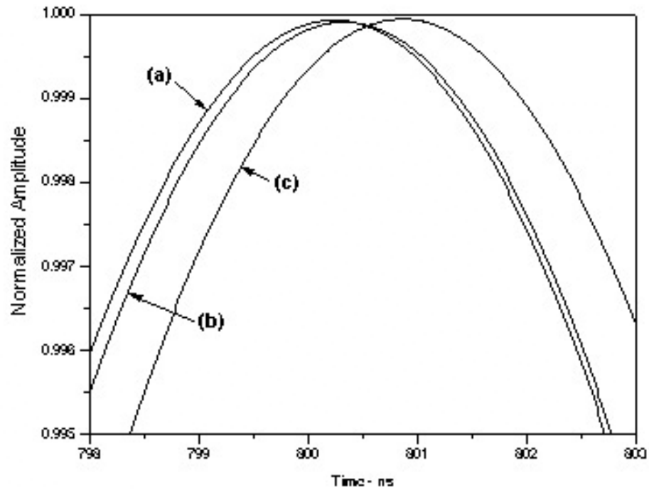
Fig. 9 – Detailed representation of the signal peak, after propagation through the setup in Fig. 6 with different lengths L_2 of the intermediate (“normal-sized”) waveguide and with different carrier frequencies f_w : (a) L_2 = 101\text{mm} , and 5.574\text{GHz} ; (b) L_2 = 501\text{mm} , and 3:5795\text{GHz} ; (c) again L_2 = 101\text{mm} , but f_w = 5.58945\text{GHz} .
