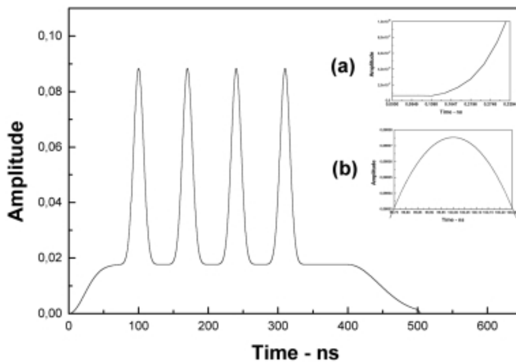
Fig. 13 – Envelope of the signal in Fig. 11 after having propagated through the undersized waveguide in Fig. 10. Inset (a) shows in detail the initial part (in time) of such arriving signal, while inset (b) shows the peak of the gaussian pulse that had been initially modulated by centering it at t = 100 ns (one can see that its propagation took zero time).
