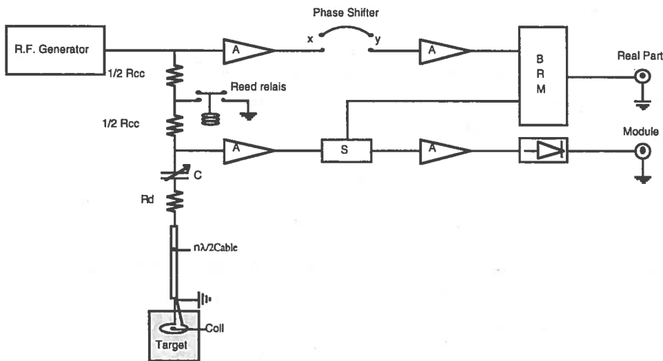
FIG. 3 – The NMR circuit to measure the polarization. The following elements are indicated: constant current resistor Rcc, tunable capacitor C, dumping resistor Rd, amplifiers A, splitter S and phase sensitive detector BRM. The real part and the module of the output signal are also indicated.
