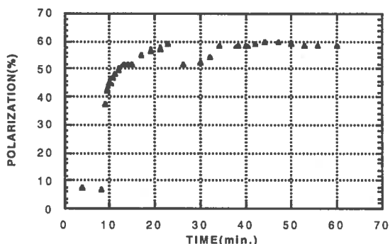
FIG. 7 – The DNP polarization at 2.0 0 K and 139.57 GHz; the small bump at t=25' indicates the helium filling on the VTI.
