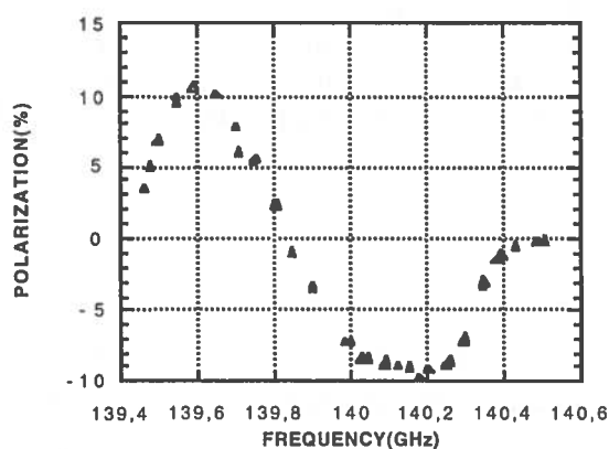
FIG. 6 – The DNP at 4.2 \text{ }^{\circ}\text{K} as a function of the MW frequency.
