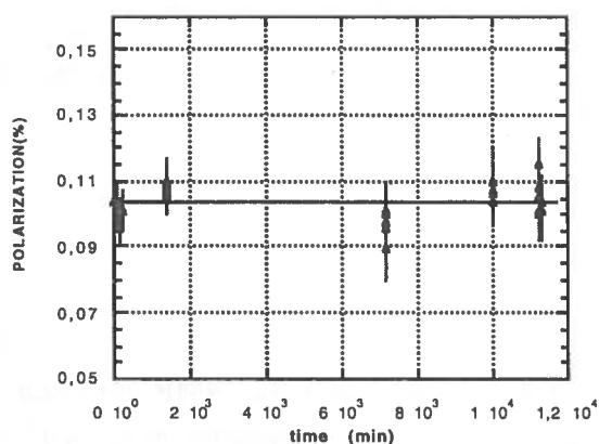
FIG. 5 – The TE polarization at 4.2 \text{ }^{\circ}\text{K} measured in one week period.
