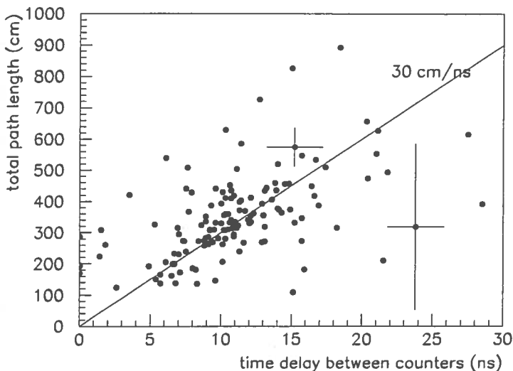
Figure 3: Total path length (see text) versus time delay \Delta t = (T_3 - T_2) between scintillation counter hits in the bottom plane. Only the 168 events for which |z_v^w - z_v^s| < 50 \text{ cm} are included. The large spread around the central line is due to the combined uncertainty in the total path length and timing reconstruction. As an example, error bars are drawn for two events. For three events, T_2 is missing and \Delta t = 0
