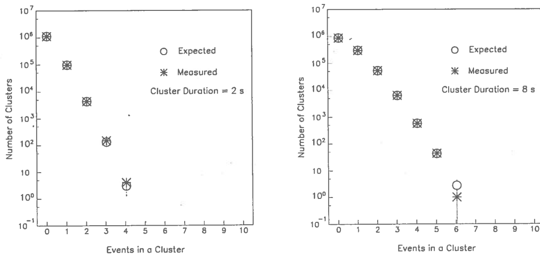
Figure 4: Observed and predicted number of event clusters vs cluster multiplicity for time intervals of 2 seconds (left) and 8 seconds (right) during the one-year monitoring period. A similar plot for the ERP system also indicates no deviation from the Poisson expectation.
