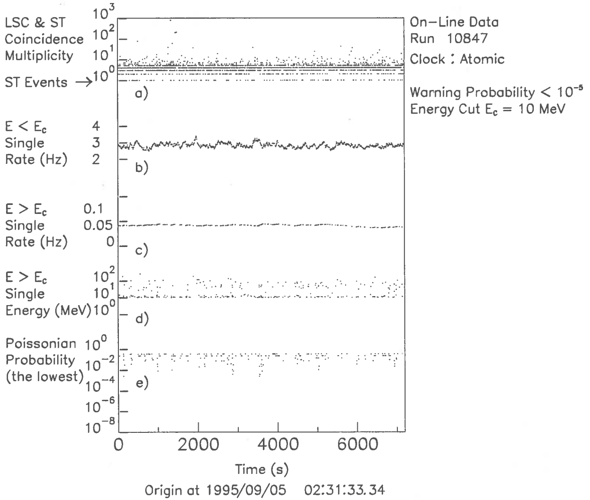
Figure 1: The display of the PHRASE supernova monitor program. LSC means "Liquid Scintillation Counter" and ST "Streamer Tubes".
