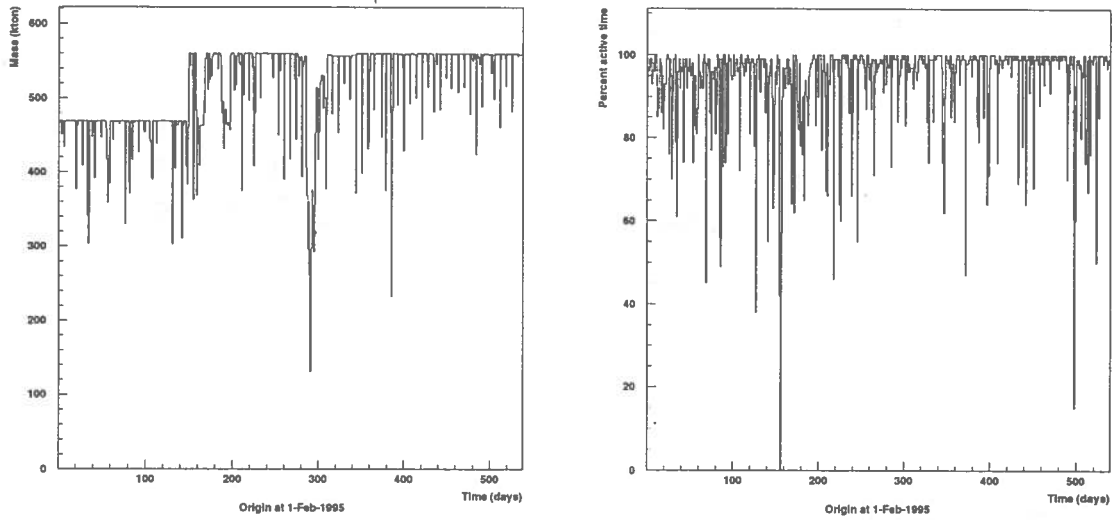
Figure 2: Liquid scintillator active mass (left) and percentage of time in each day that the search was active (right) during the one and a half year period
