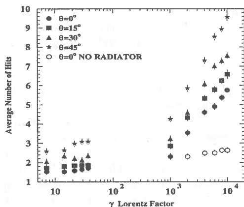
Figure 1. Average total number of hits for various values of the \gamma factor : dots: 0° incident beam angle; open circles: 0° beam angle without radiator; squares: 15° beam angle; triangle: 30° beam angle; stars: 45° beam angle.
