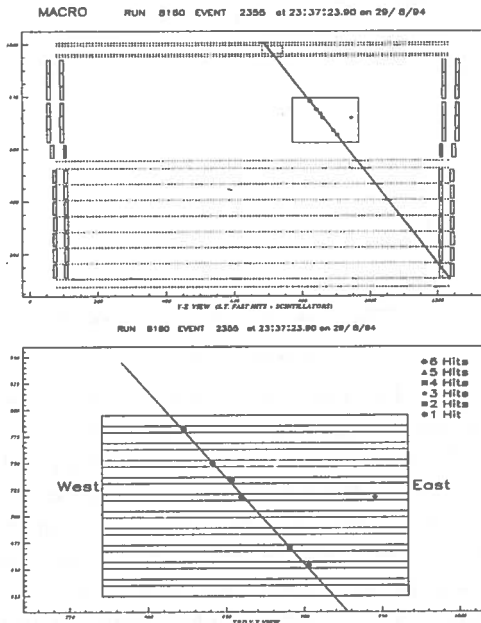
Figure 2. On-line display of a typical single muon track crossing MACRO and the TRD (upper part). In the lower part an enlarged view of the TRD is shown.
