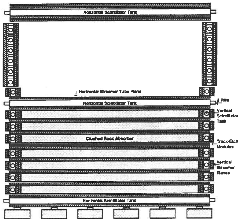
Figure 2: A single MACRO supermodule in cross sectional view. It is 12.6 m long, 12 m wide and 9.6 m high.
