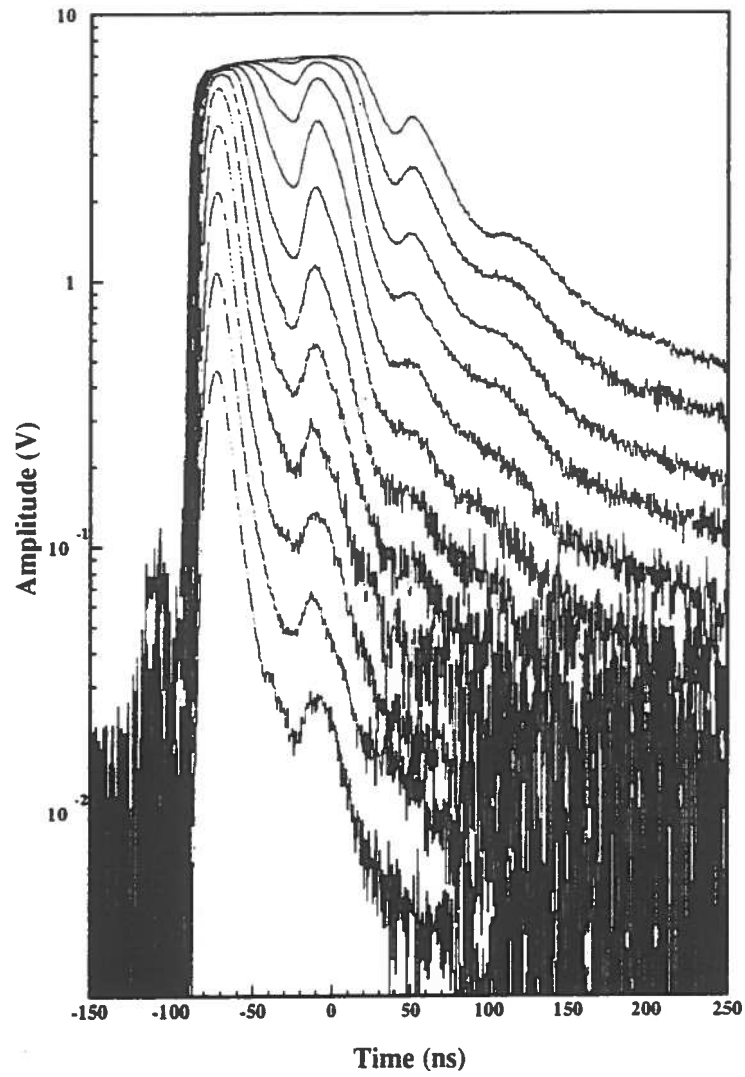
Figure 4: Photomultiplier waveforms recorded at various laser light intensities. The first optical reflection is clearly visible. At higher intensities the second and third reflections become apparent, as do the effects of pulse saturation. A vertical muon corresponds to the pulse peaking at about 1 V.
