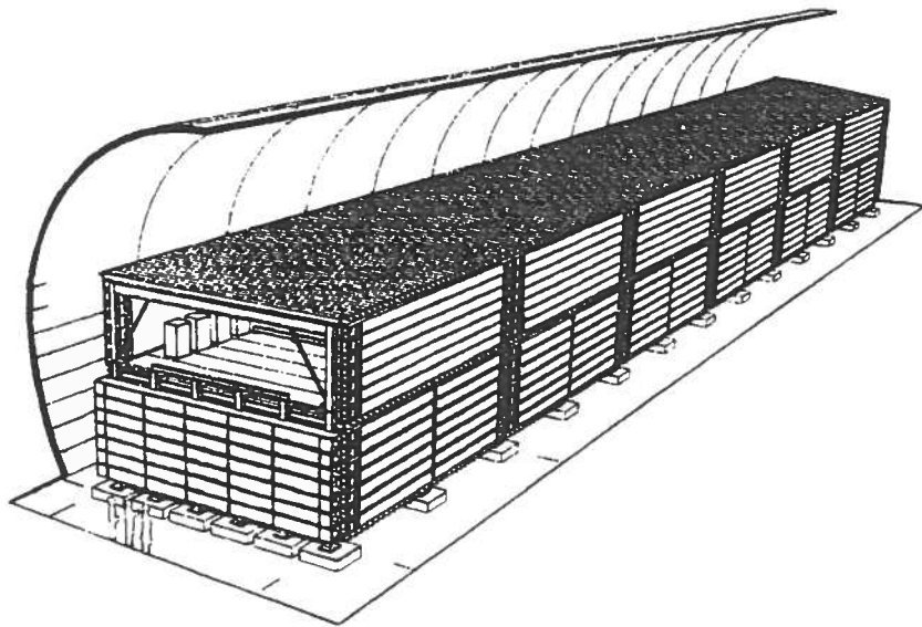
Figure 1: The complete MACRO detector in perspective view. It is 76.5 m long, 12 m wide, and 9.6 m high.
