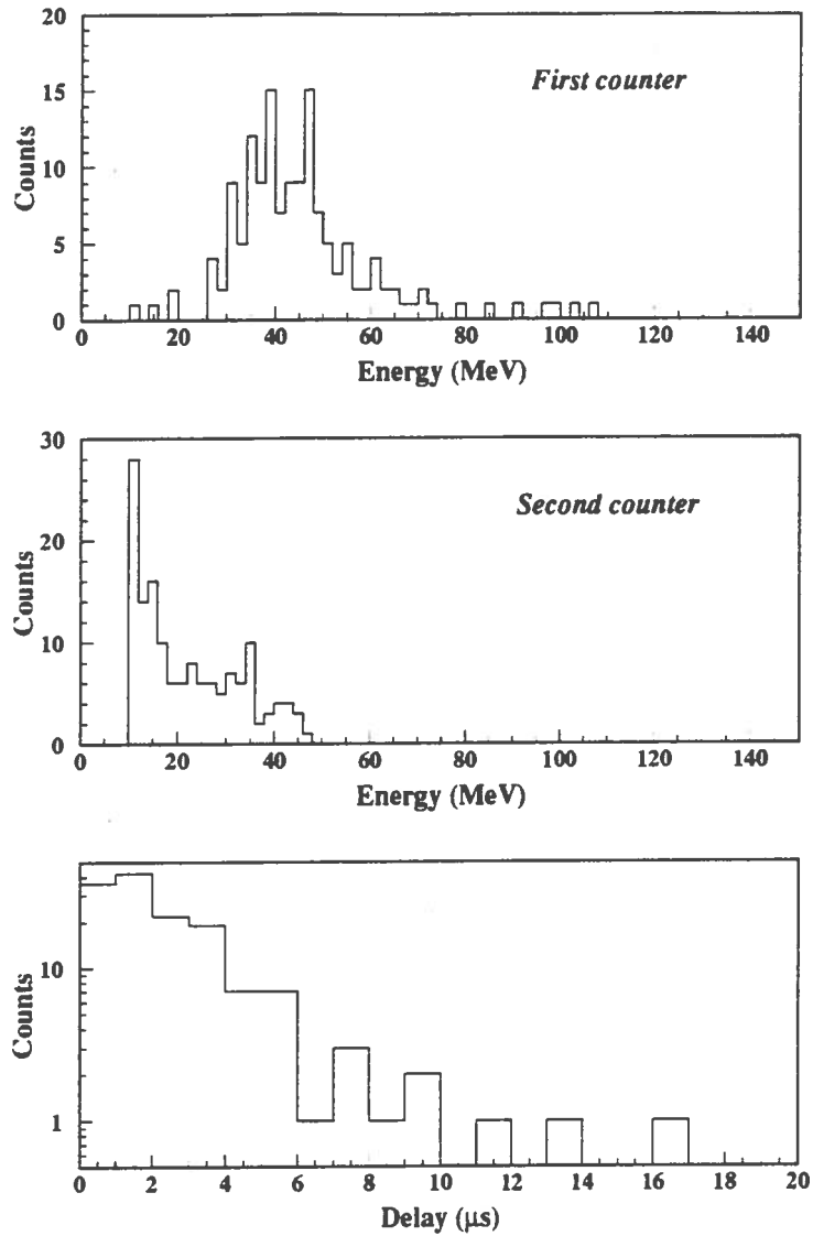
Figure 13: Energy loss and timing measurements for the downward-going PHRASE candidates. Losses in the first scintillator counter are consistent with the Landau distribution for minimum ionizing particles, while in the second counter there is a cutoff at \approx 50 MeV. The timing distribution (the delay between the first and second counters signals) is consistent with a few \mu s lifetime particle decay.
