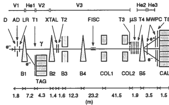
Fig. 2. Experimental set-up, seen from above. The distances are not to scale.
