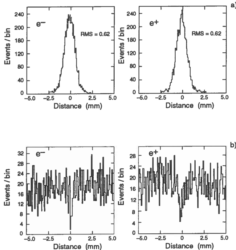
Fig. 3. Distribution of distances between extrapolated positions from \mu S and MWPC, for e^- and e^+ : a) good choice, b) bad choice.
