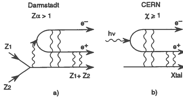
Fig. 1. Induced pair creation in strong fields.
