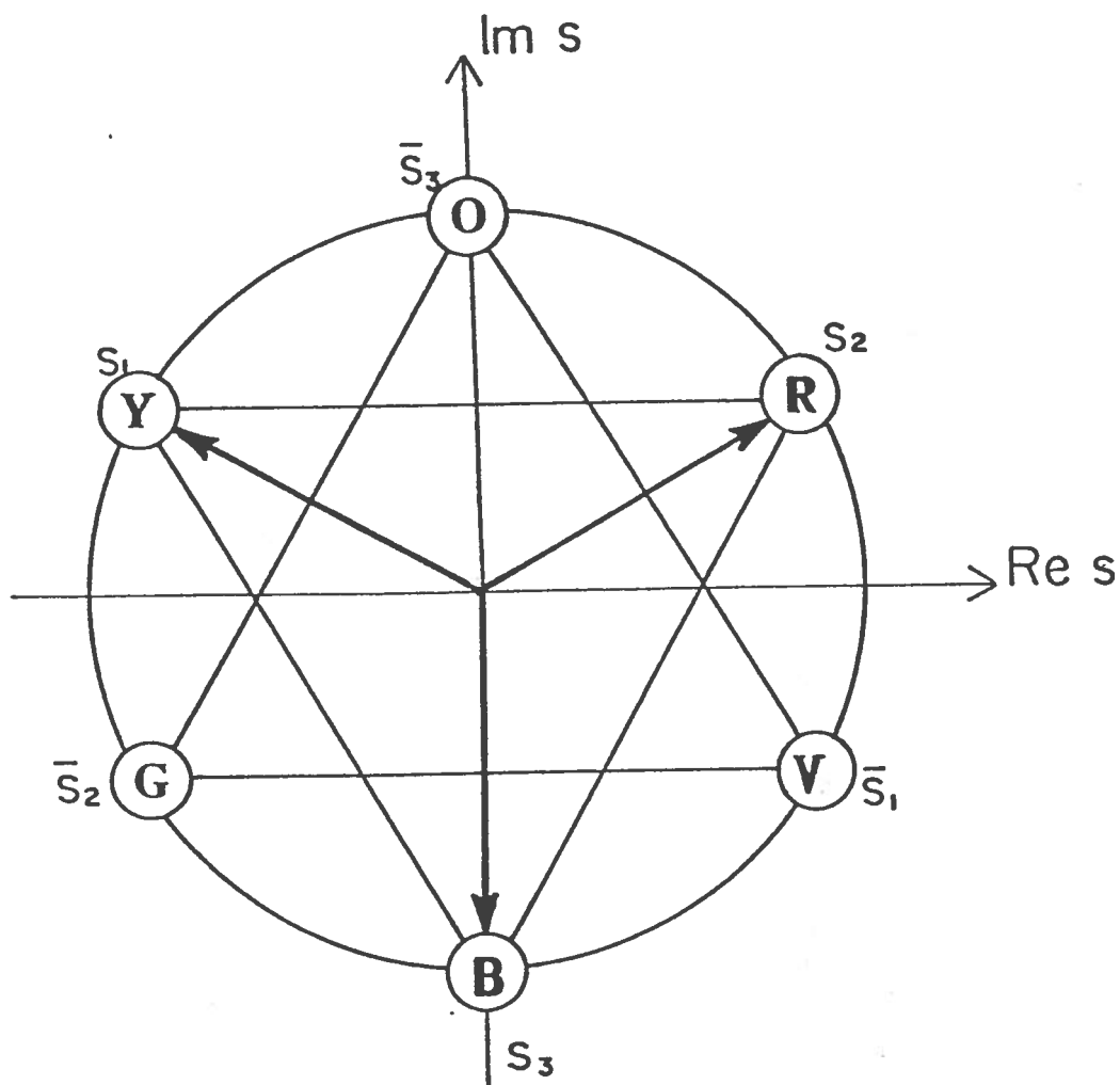
Fig. 1 - "Coloured" quarks and their strong charge - This scheme represents the complex plane 3,12,13 of the sign s of the quark strong-charges g_j in a hadron. These strong charges can have three signs, instead of two as in the case of the ordinary electric charge e . They can be represented, for instance, by s_1 = (i - \sqrt{3})/2 ; s_2 = (i + \sqrt{3})/2 ; s_3 = -i , which correspond to the arrows separated by 120^\circ angles. The corresponding anti-quarks will be endowed with strong charges carrying the complex conjugate signs \bar{s}_1, \bar{s}_2, \bar{s}_3 . The three quarks are represented by the "yellow" (Y), "red" (R) and "blue" (B) circles; the three anti-quarks by the "violet" (V), "green" (G) and "orange" (O) circles. The latter are complementary to the former corresponding colors. Since in real particles the inter-quark forces are saturated, hadrons are white. The white colour can be obtained either with three-quark structures, by the combinations YRB or VGO (as it happens in baryons and antibaryons, respectively), or with two-quark structures, by the combinations YV or RG or BO [which are actually quark-antiquark combinations], as it happens in mesons and their antiparticles. See also note 11 .
