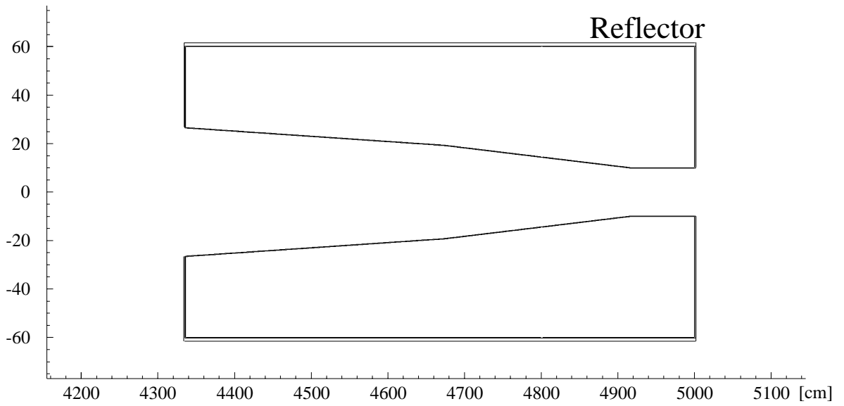
Figure 16: Cross section of the conductor in horn and reflector.
