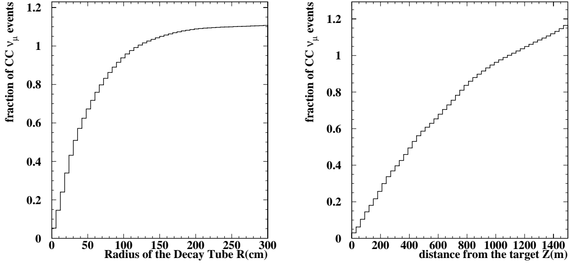
Figure 11: Cumulative radial (left) and longitudinal (right) distribution of the decay points of parent hadrons which produce \nu_\mu events at Gran Sasso, normalised to the NGS design values R = 122.5 cm and Z = 1100 m.
