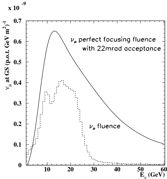
Figure 9: Comparison of 'perfect focusing' with the \nu_\mu fluence at Gran Sasso.
