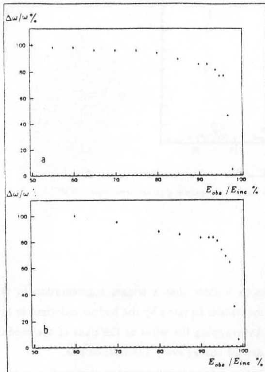
Fig.15 Solid angle fraction over which an electron can hit the HPC, so that a given fraction of its energy is measured by the module trigger system (a) and by the sector trigger system (b)
