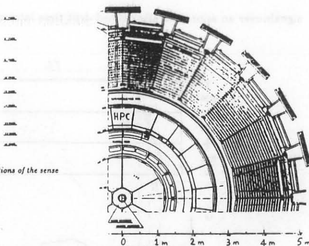
Fig.2 Cross section of the DELPHI detector.
