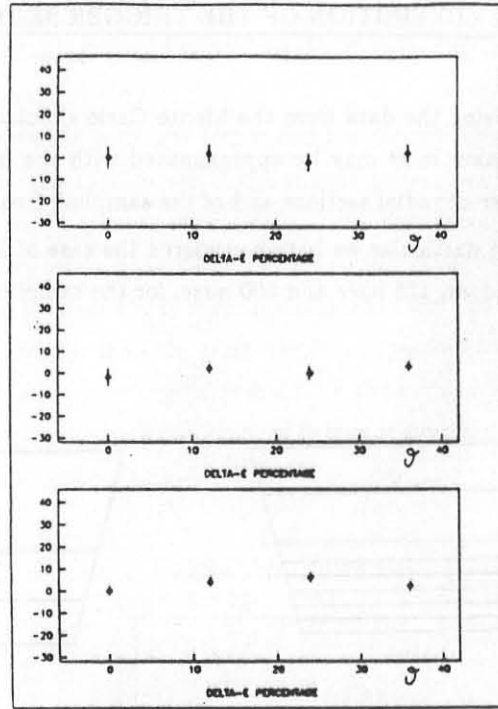
Fig.9b Difference (in percentage) between the energies released in two contiguous trigger sectors by electrons having the sector boundary as incidence direction: 9 radial sections, 125 nsec sampling period.
