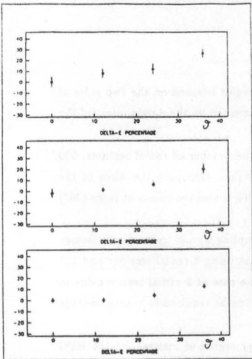
Fig.9c Difference (in percentage) between the energies released in two contiguous trigger sectors by electrons having the sector boundary as incidence direction: 8 radial sections, 125 nsec sampling period.
