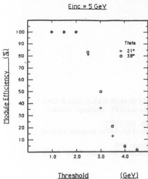
Fig.14 Trigger efficiency as a function of the applied energy threshold: the 21° direction crosses the boundary between the 1 st and the 2 nd module, the 38° direction crosses the boundary between the 2 nd and the 3 rd module (module scheme).
