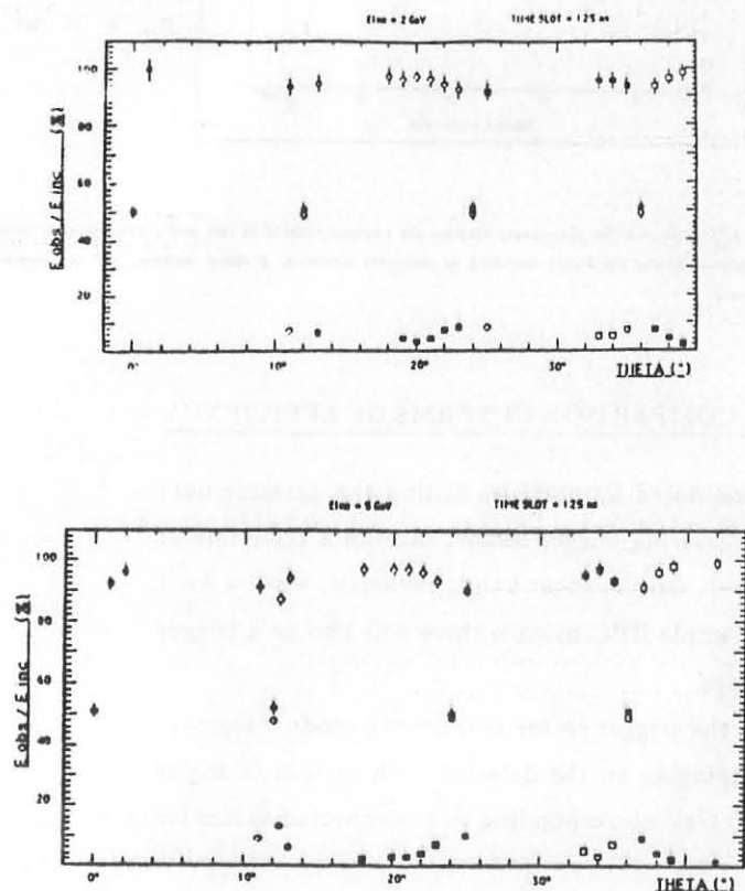
Fig. 11 Incident energy fraction observed in each trigger sector, as a function of the incidence angle ( \circ \equiv 1^{st} sector; \diamond \equiv 2^{nd} sector; \triangle \equiv 3^{rd} sector; \square \equiv 4^{th} sector). The sectors are defined by means of three radial sections.
