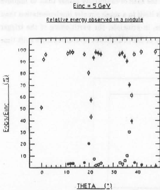
Fig.13 Incident energy fraction observed in each module, as a function of the incidence angle ( \theta \equiv 1^{\text{st}} module; \bullet \equiv 2^{\text{nd}} module; \square \equiv 3^{\text{rd}} module).
