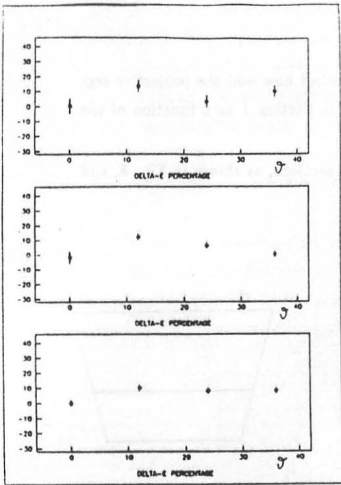
Fig.9a Difference (in percentage) between the energies released in two contiguous trigger sectors by electrons having the sector boundary as incidence direction: 8 radial sections, 125 nsec sampling period.
