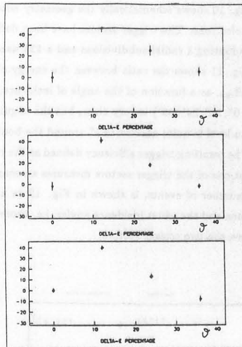
Fig.9f Difference (in percentage) between the energies released in two contiguous trigger sectors by electrons having the sector boundary as incidence direction: 2 radial sections, 500 nsec sampling period.
