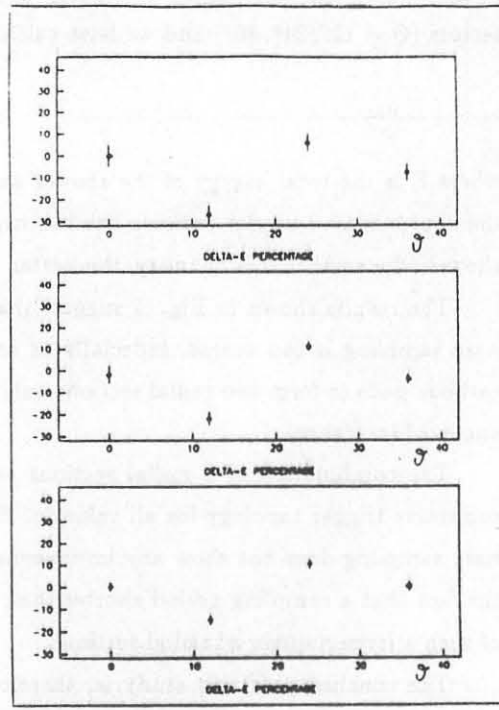
Fig.9d Difference (in percentage) between the energies released in two contiguous trigger sectors by electrons having the sector boundary as incidence direction: 8 radial sections, 500 nsec sampling period.
