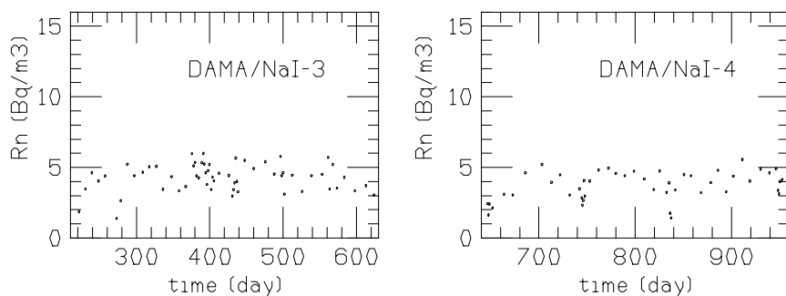
Figure 5: Behaviour of the environmental Radon inside the inner part of the barrack from which – as mentioned in the text – the detectors are excluded. The time scale starts from January, 1 st 1997.
