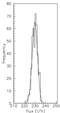
Figure 4: Distribution of the HP Nitrogen flux during both the DAMA/NaI-3 and DAMA/NaI-4 running periods.
