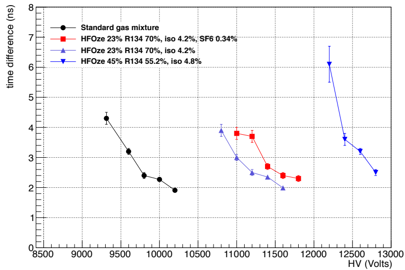
Figure 14: Difference between the time over threshold of two RPCs vs effective HV for different mixtures composed by isobutane, R134a, HFO1234ze with and without SF_6 . To get the real time resolution the values should be divided for something of the order of \sqrt{2} .
