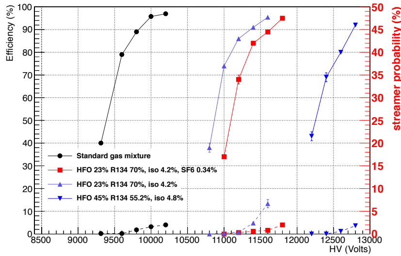
Figure 12: Efficiency and streamer probability vs effective HV for different mixtures composed by isobutane, R134a, HFO1234ze with and without SF_6 . Streamer probability is indicated with dashed line and the scale is on the right y axis
