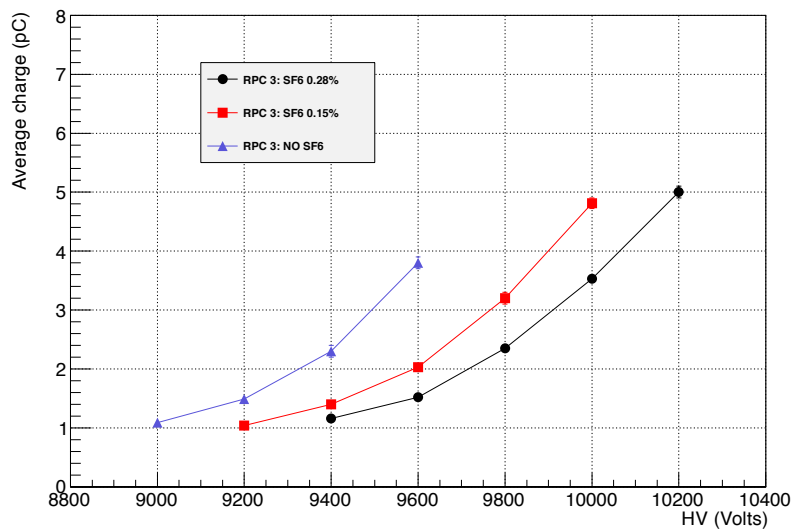
Figure 7: Integrated induced charge vs effective HV for a mixture composed by 4.5 % of isobutane, about 95.2 % of R134a and varying the amount of SF_6 between 0 and 0.28 %. The amount of R134a is adjust accordingly
