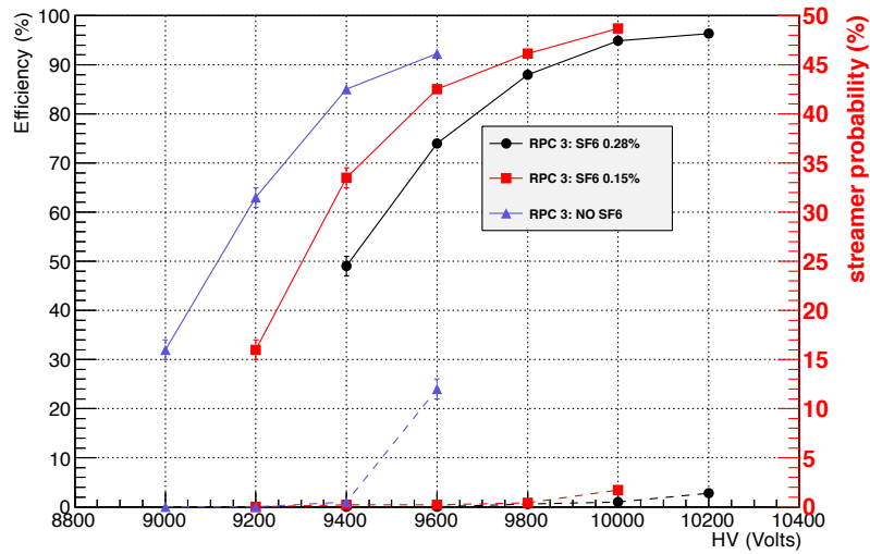
Figure 6: Efficiency and streamer probability vs effective HV for a mixture composed by 4.5 % of isobutane, about 95.2 % of R134a and varying the amount of SF_6 between 0 and 0.28 %. The amount of R134a is adjust accordingly. Streamer probability is indicate with dashed line and the scale is on the right y axis
