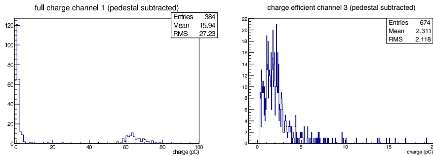
Figure 5: Left: Typical distribution of the induced charge integrated in a 150 ns time window of the “signal region” for one of the gas mixtures tested and working in streamer mode. The peak of the streamers is clearly seen for induced charges above 20 pC. Right: induced charge distribution for the CMS standard gas mixture showing the avalanche peak
