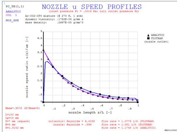
Figure 5 – Speed profiles.
