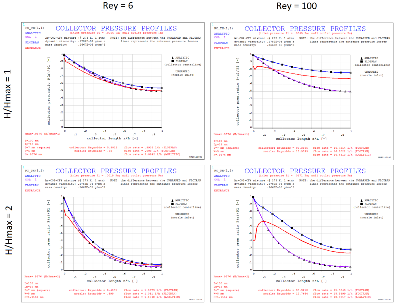
Figure 4 – Pressure profiles.
