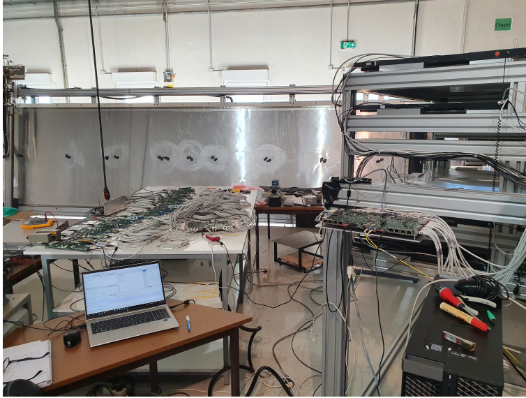
Figure 4: Read-Out board final prototypes tests at Strasbourg. Test bench simulation of one wall (16 FEC-ROB coupled to one concentrator at left and detector prototype for track reconstruction at right.
