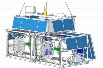
Figure 1: Layout of the SPB2 instrument, showing the two telescopes (Fluorescence and Cherenkov) and the arrangement in the gondola of the Payload
