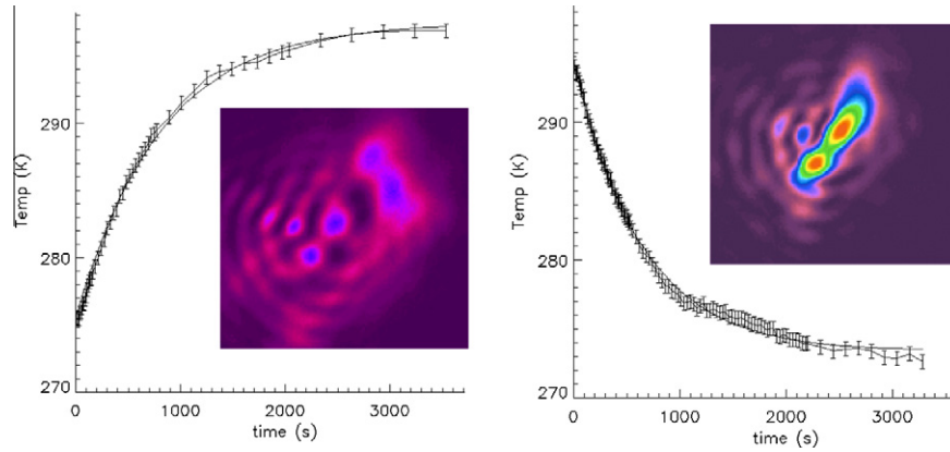
Fig. 23. Warm-up (left), cool-down (right) curves of the CCR front face and FFDPs taken at the end of the curves. Exponential fits give \tau_{CCR} = (720 \pm 80) s, \Delta T = (21.5 \pm 0.6) K.
