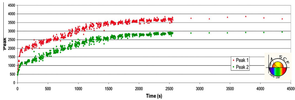
Fig. 18. GLONASS/GIOVE CCR cool-down: FFD intensity at the average velocity aberration of ILRS stations for GNSS satellites ( 25 \mu\text{rad} ) vs. time.
