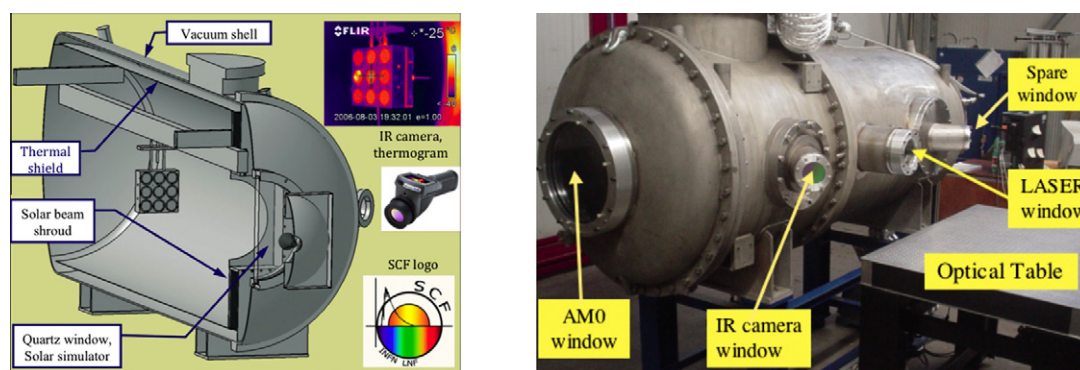
Fig. 3. Left: SCF cryostat with an Apollo/LAGEOS LRA built at LNF (Bosco et al., 2007), LRA thermogram, one IR camera and SCF logo. Right: SCF cryostat, windows and optical table for FFDP tests. The 45° and 135° ports can host windows with clear diameters up to \sim 200 mm.
