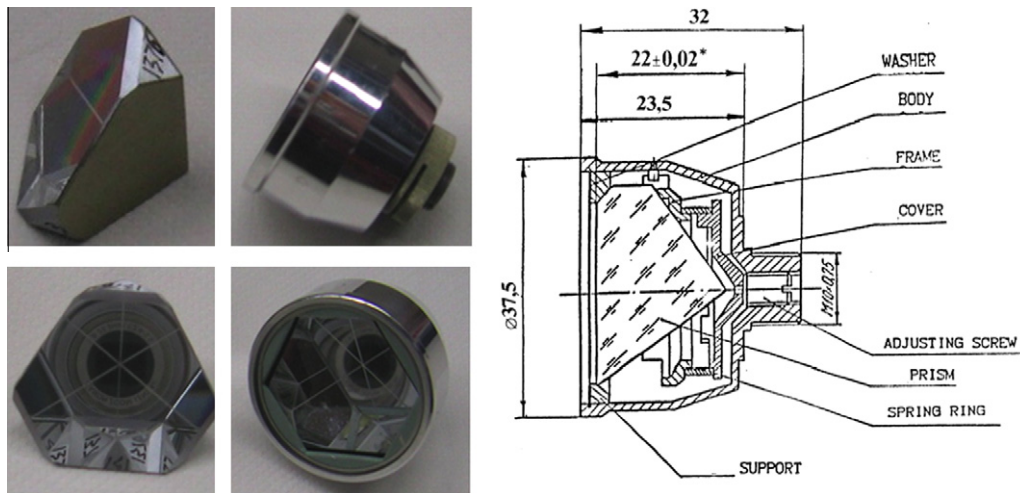
Fig. 8. The GLONASS/GPS/GIOVE CCR: bare coated CCR (left); complete CCR, mounted in its aluminum housing (center); some details of the mounting scheme (right).
