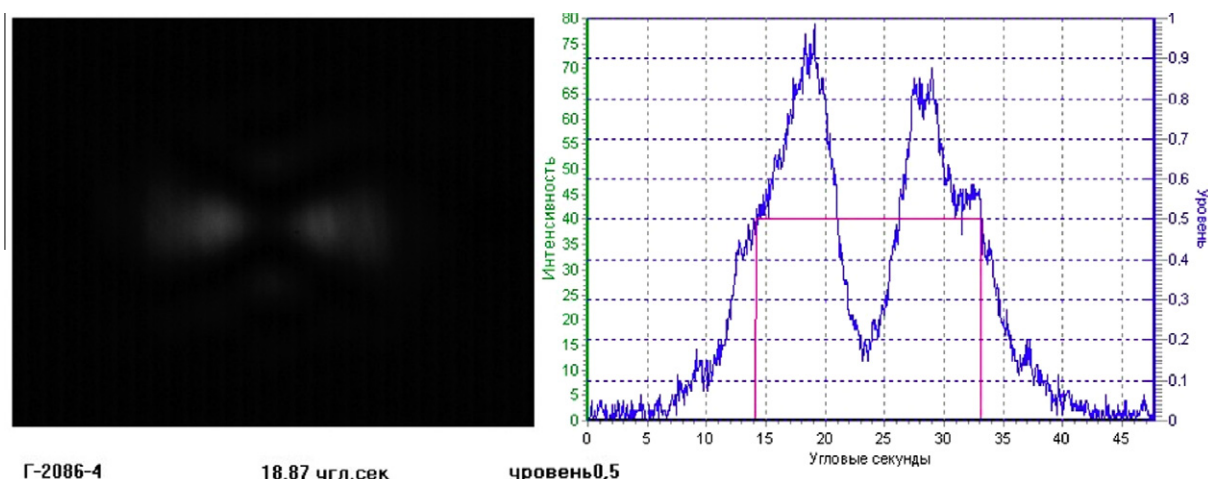
Fig. 11. FFDP angular distance measured by IPIE in arc-sec for 532 nm.
