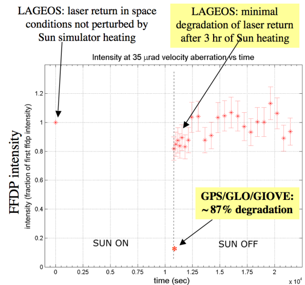
Figure 7. LAGEOS CCR: FFDP relative intensity after degradation due to SS heating. Shown is also the 87% GPS FFDP degradation reported at t \sim 3000 in Fig. 2
