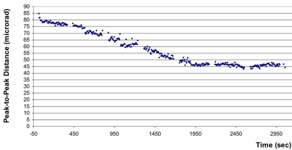
Figure 5. GPS-2 flight CCR: recovery of FFDP peak-to-peak distance up to the nominal velocity aberration of 45\text{-}50\ \mu\text{rad} , after degradation due to SS heating
