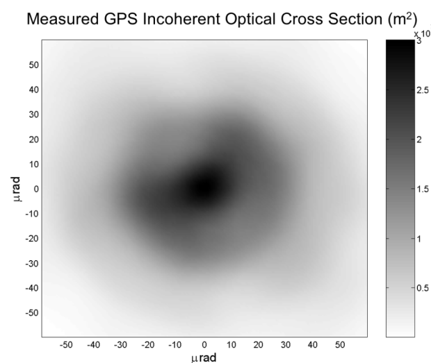
Figure 20. GPS-2 flight array: OCS measured at 532 in the velocity aberration (FFDP) plane. Vertical scale is 0\text{--}3 \times 10^7 \text{ m}^2 , horizontal scale is [-60, +60] \mu\text{rad}
