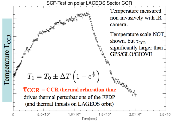
Figure 8. LAGEOS CCR heating and cooling curves. Horizontal scale is 0-2.5 \times 10^4 sec
