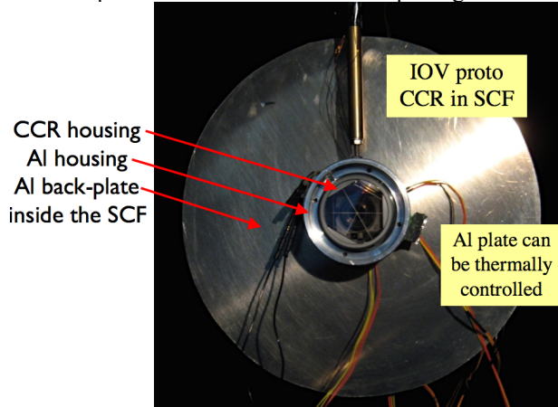
Figure 13. IOV CCR inside the SCF for the GCO test
