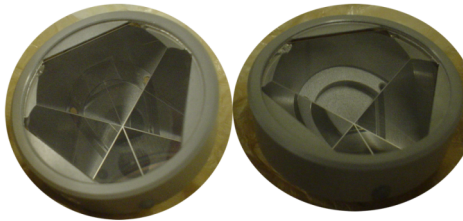
Figure 11. Uncoated IOV CCR. Left: camera taking photo at angle \sim 17^\circ is still barely visible. Right: at angle > 17^\circ camera is not visible due to optical BT
