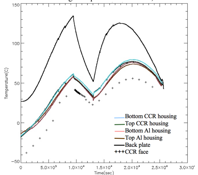
Figure 14. Temperatures of the IOV CCR package during the GCO. The horizontal scale is 0-3 \times 10^4 sec
