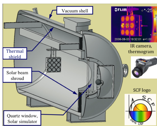
Figure 18. SCF cryostat with Apollo/LAGEOS array built at LNF, IR thermogram, IR camera, SCF logo
