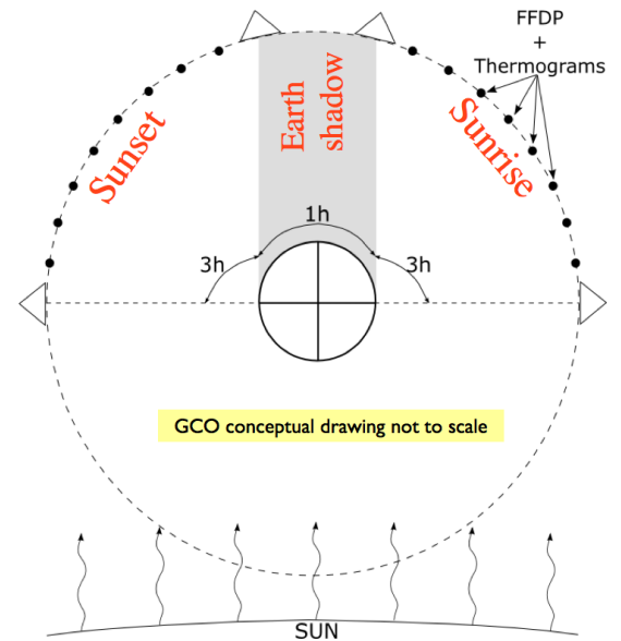
Figure 10. Galileo GCO: Sunrise (3 hr)–eclipse (1 hr)–sunset (3 hr) sequence and concurrent measurements
