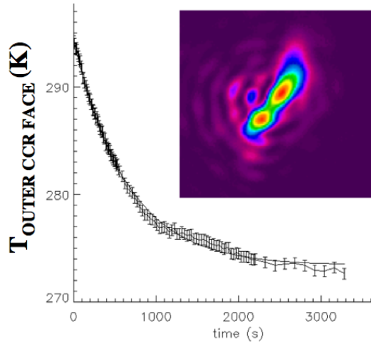
Figure 4. GPS-2 flight CCR: thermal relaxation after degradation due to SS heating. Inset: FFDP at t \sim 3000 , with peaks at the nominal 45\text{-}50\ \mu\text{rad} distance
