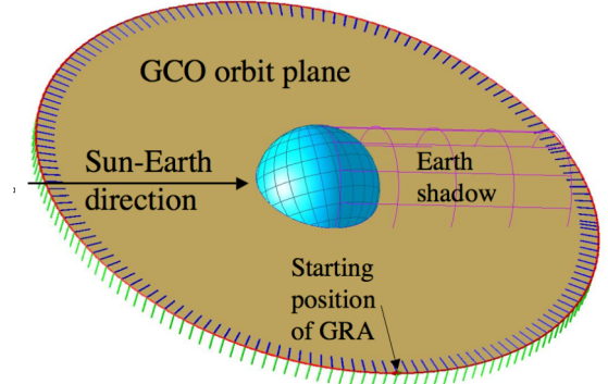
Figure 9. Drawing of the GNSS Critical half-Orbit (GCO) test of the SCF-Test/Revision-ETRUSCO-2
