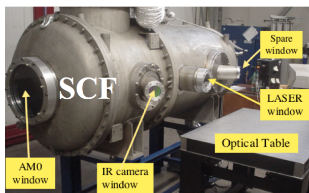
Figure 19. SCF cryostat and its windows.
