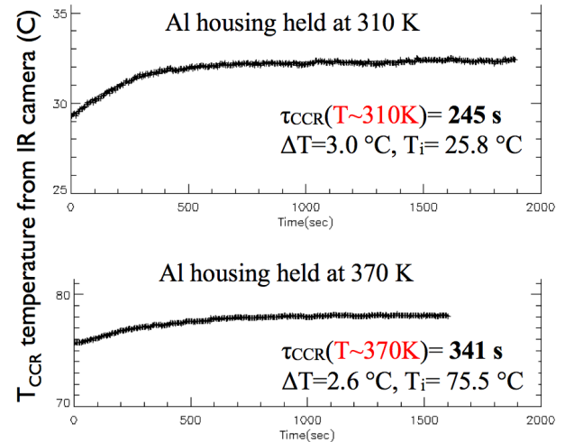
Figure 17. IOV CCR: measurement of the thermal relaxation time at T_B = 310 K and 370 K
