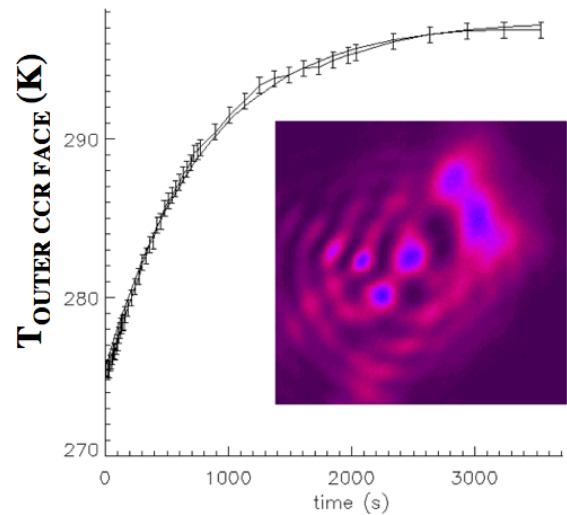
Figure 2. GPS-2 flight CCR: heating during exposure to the SS. Inset: FFDP at t \sim 3000
