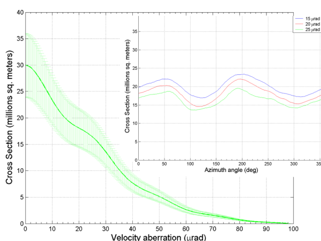
Figure 21. GPS-2 flight array: azimuth-averaged OCS vs. velocity aberration. Inset: OCS at three velocity aberrations vs. azimuth, counted anticlockwise
