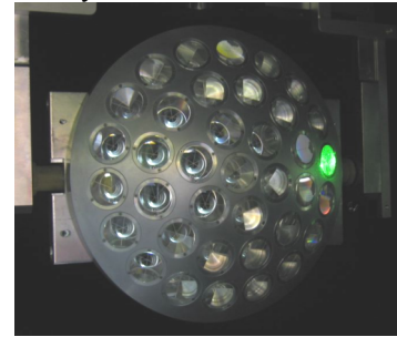
Figure 6. LAGEOS Sector engineering model property of NASA-GSFC SCF-Tested in Frascati
