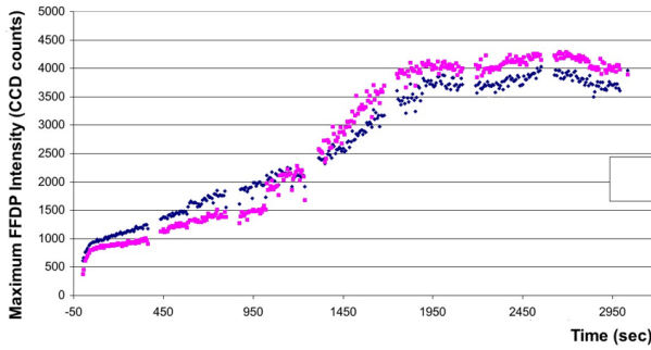
Figure 3. GPS-2 flight CCR: FFDP intensity recovery when SS heating is turned off at t = 0
