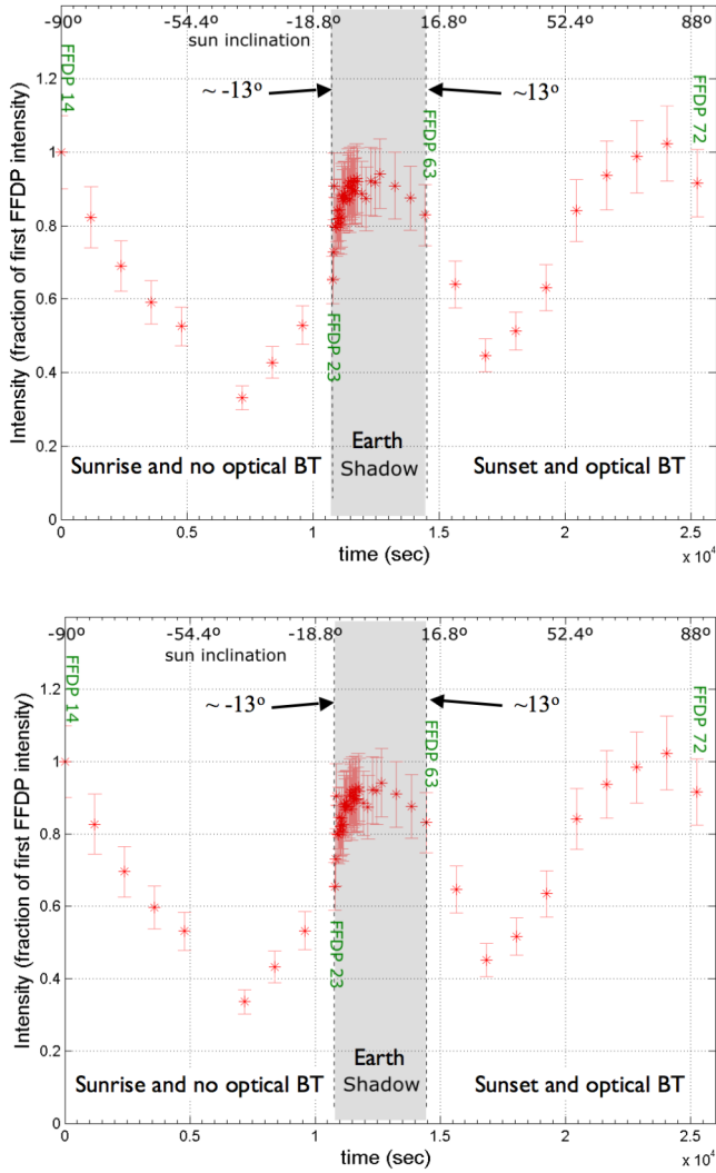
Figure 15. FFDP relative intensity of the IOV CCR during the GCO at 24 \mu\text{rad} (top plot) and in the (22-26) \mu\text{rad} range (bottom plot) of the velocity aberration. The horizontal scales are 0-2.7 \times 10^4 sec
