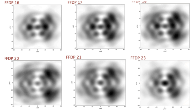
Figure 16. IOV CCR: FFDP relative intensity during the GCO. FFDP scales are [-60, +60] \mu\text{rad}
