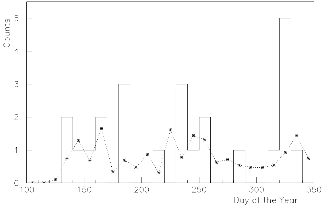
Figure 4. Number of coincidences n_c (solid line) and the average number \bar{n}_a of accidentals (dashed line) as a function of the day of the year, in 10-days bins.
