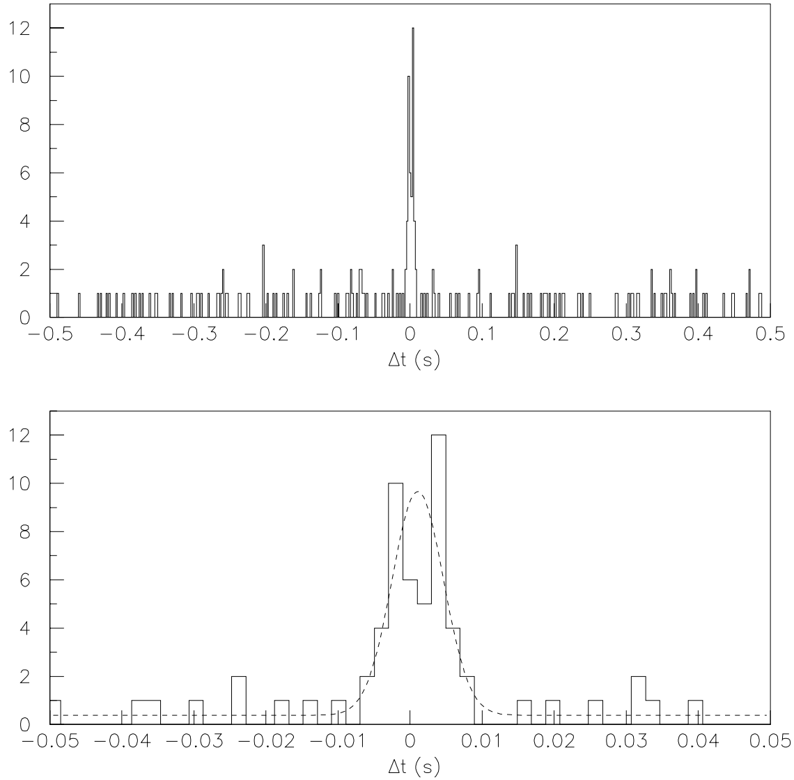
Figure 2. The distribution of the observed delays between the signal of the cosmic ray showers and the corresponding EXPLORER events. The distribution can be fitted with a constant (accidentals) plus a gaussian, giving \sigma = 3.6 \pm 0.5 ms. The lower graph is a zoom of the upper one.
