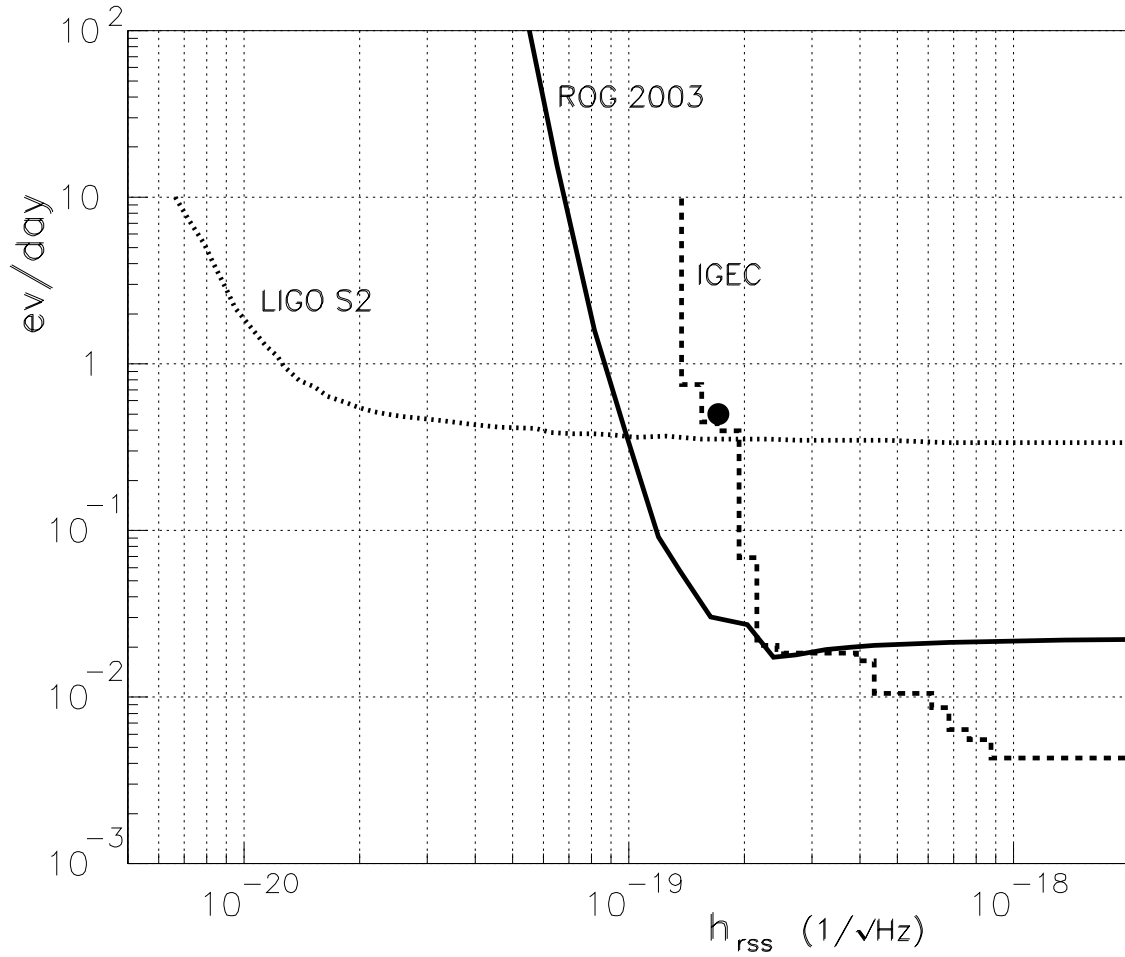
Figure 6. Upper limit (at 95 %) on the rate of events arriving on Earth as a function of h_{rss} , assuming gaussian-shaped bursts with \tau = 0.1 ms. The LIGO and IGEC curves are from fig.14 of ref.[6]. The large point represents roughly what could have been the rate deduced [21] from ours 2001 results.
