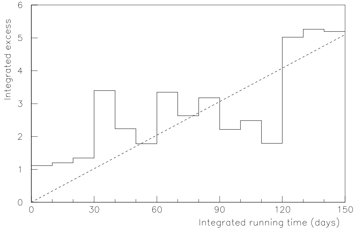
Figure 5. Excess of coincidences versus the integrated running time (solid line) and a linear fit (dashed line) giving a slope of \simeq 0.034 excess/day.
