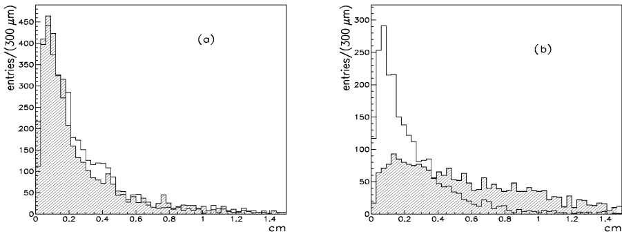
Fig. 8. Distributions of the impact parameter for Monte Carlo data, after reconstruction, in the two cases: (a) production of an uncorrelated \pi^- p pair from the K^- vertex, and (b) production of \Sigma^- and p from the decay vertex, and following \Sigma^- decay. The open histograms correspond to the proton, and the hatched ones to the \pi^- case.
