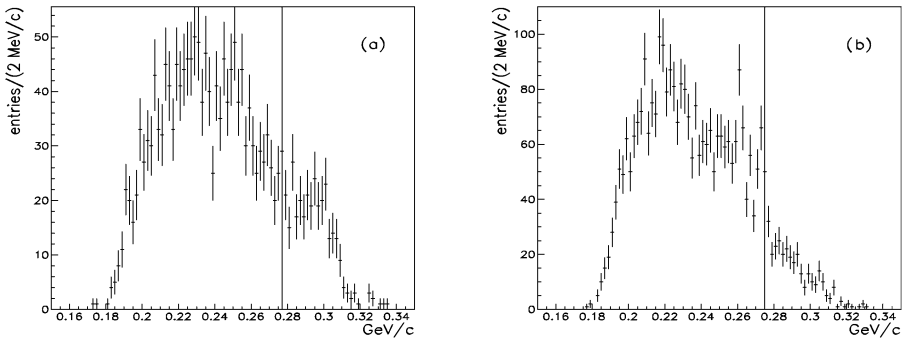
Fig. 4. Momentum spectrum of \pi^- in coincidence with a proton: {}^6\text{Li} (a) and {}^{12}\text{C} (b). The vertical lines indicate the limit for \Lambda hyperfragments production. The narrow peaks in (b) are due to the formation of the ground state and the 10 MeV excited state of {}^1_{\Lambda}\text{C} .
