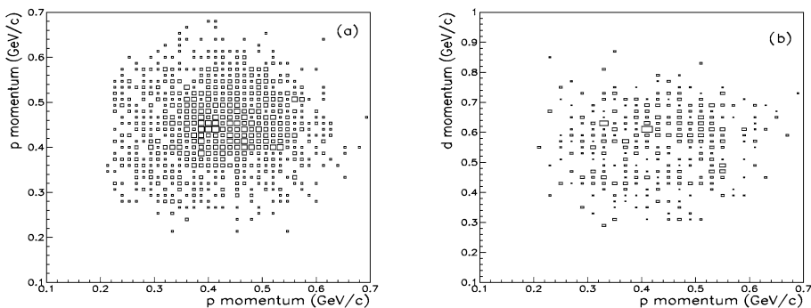
Fig. 2. Two-dimensional scatter plot of the proton momentum versus (a) a second proton track or (b) a deuteron track, both recognized by specific energy loss, and coming from a common vertex in {}^6\text{Li} targets.
