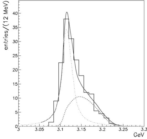
Fig. 6. Missing mass spectrum obtained in the hypothesis of the reaction K^- + {}^4\text{He} \rightarrow X + p , for data with reconstructed vertices on {}^6\text{Li} targets; the {}^4\text{He} nucleus is assumed to be at rest and not subject to any Fermi motion. The dashed curve is a background shape fitting the analogous spectrum obtained for {}^{12}\text{C} under the same hypothesis, adapted to the tail of the {}^6\text{Li} distribution; the sum of this contribution to a Gaussian fitting the peak (dotted line), properly weighted, gives the solid line fitting the distribution.
