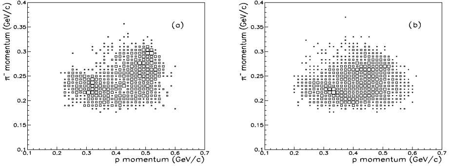
Fig. 3. Two-dimensional plot of the \pi^- momentum versus the proton momentum from {}^6\text{Li} (a) and {}^{12}\text{C} (b).
