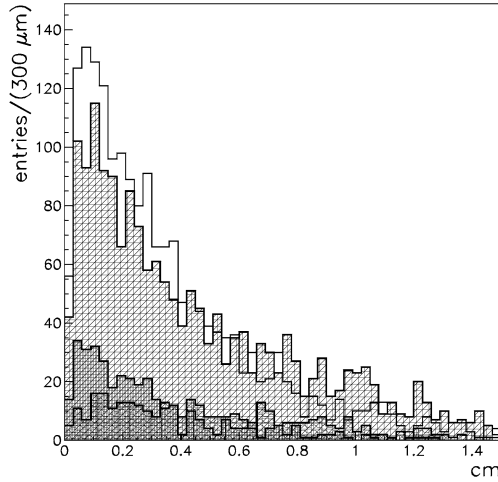
Fig. 9. Distribution of the impact parameter for protons (white histogram) and pions (hatched histogram) following the interaction of a K^- in the {}^6\text{Li} targets. The vertical hatched histogram and the wavy one correspond to the proton and \pi^- impact parameter distributions for events with p_{\pi^-} > 275 \text{ MeV}/c .
