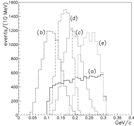
Fig. 7. Monte Carlo momentum spectra for the \pi^- coming from a hyperon decay together with a \sim 500 MeV/c proton in the following reactions: (a) black solid line: K^- + d \rightarrow p + \Sigma^- ; (b) dashed line: K^- + {}^4\text{He} \rightarrow S^0 + p , with the following S^0 \rightarrow \Lambda nn decay; (c) dotted line: K^- + {}^4\text{He} \rightarrow S^0 + p , with the following S^0 \rightarrow \Sigma^- np decay; (d) dot-dashed line: K^- + {}^4\text{He} \rightarrow S^0 + p , with the following S^0 \rightarrow \Sigma^- np decay and \Sigma^- p \rightarrow \Lambda n conversion; (e) grey solid line: K^- + {}^4\text{He} \rightarrow S^0 + p , with the following S^0 \rightarrow \Sigma^- d decay. The spectra show the pure kinematics of the reaction without any filtering through the apparatus acceptance and reconstruction. The hyperon is always assumed to decay in flight. The {}^4\text{He} and d target nuclei are assumed to be at rest and not embedded inside a composite nucleus. When they are endowed with a Fermi momentum, which depends on the target nucleus, the distributions are moved toward higher momenta and their edges are more smeared.
