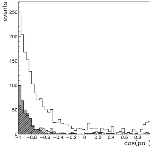
Fig. 10. Distribution of the angle between a proton and a \pi^- track following the interaction of a K^- in the {}^6\text{Li} targets: the white histogram is for all events, the shaded one for events with the pion momentum larger than 275 MeV/c, the hatched one for events with the proton momentum in the window (275–350) MeV/c. All the distributions are acceptance corrected and normalized to the number of selected events in each sample.
