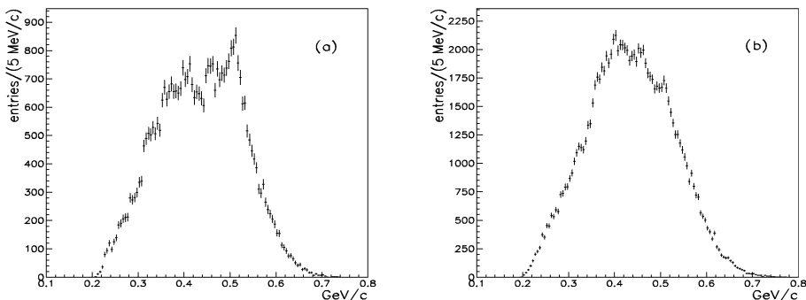
Fig. 1. Inclusive proton spectra measured following the K^- capture at rest from ^6\text{Li} (a) and ^{12}\text{C} (b).
