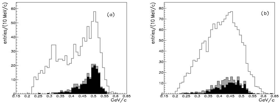
Fig. 5. Momentum spectrum of protons in coincidence with a \pi^- : (a) {}^6\text{Li} , (b) {}^{12}\text{C} . The shaded spectra are obtained with the condition of a \pi^- momentum larger than 275 MeV/c for {}^6\text{Li} and 272 MeV/c for {}^{12}\text{C} . The black spectra are obtained with the further condition of an angular correlation \cos\theta_{(\pi^-p)} < -0.8 .
