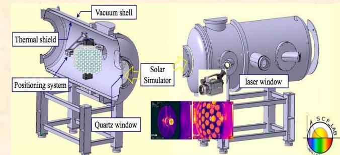
Schematic view of SCF cryostat with: IR picture of the LAGEOS Sector, IR camera and SCF_LAB logo.
