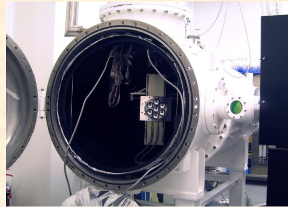
GRA-H installed on the roto-translation positioning and thermal control system in the SCF (IR window in green color on the right).
