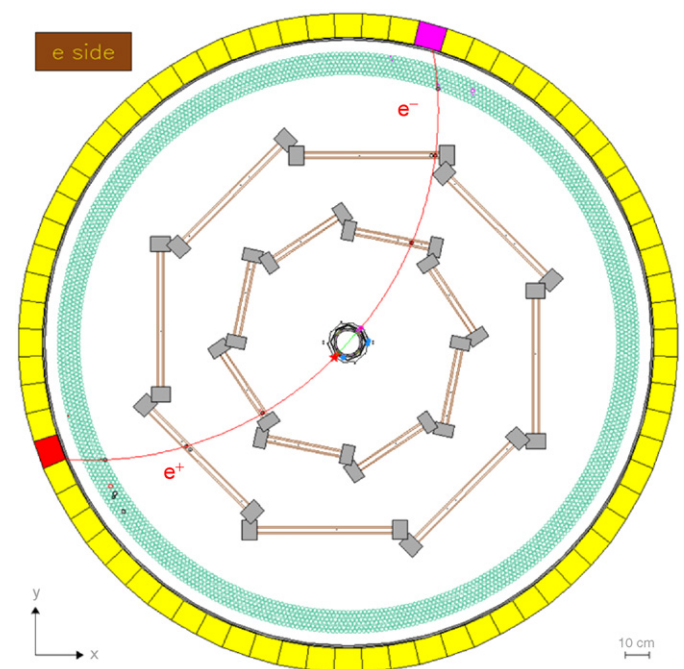
Fig. 2. Highly elastic Bhabha event e^+e^- \rightarrow e^+e^- recorded by the FINUDA spectrometer. The reconstructed momenta of the e^+ and e^- track are 512 and 492 MeV/ c , respectively.
