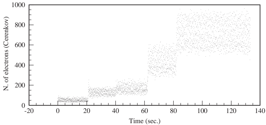
Fig. 24. Measurement of number of particles per bunch by using the Cherenkov counter (after calibration with Calorimeter 2) as a function of time. The multiplicity during the run was increased by opening the collimators.
