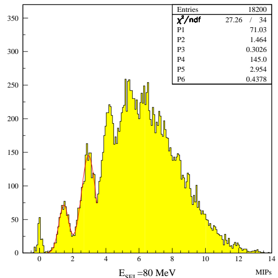
Fig. 16. Energy deposited in Calorimeter 1 for E_{\text{sel}} = 80 MeV after gain equalization. The Gaussian fit to the first and second electron peak is also shown.
