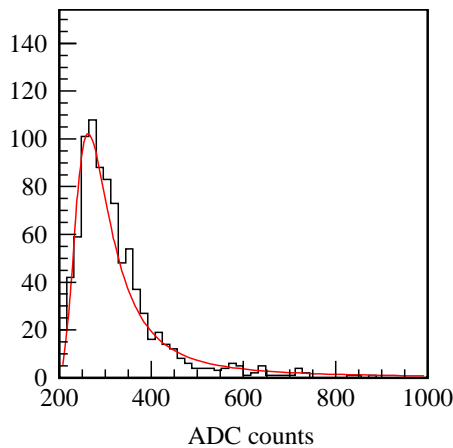
Fig. 15. Calorimeter 1: example of 1 channel cosmoics spectrum with superimposed Landau fit.
