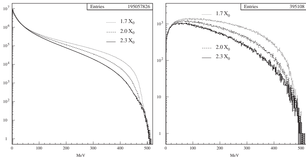
Fig. 8. Electron energy distributions: (a) without angular cut and (b) for \theta \leq 4 mrad, for the three different degrader target thicknesses, at the exit of the first slit collimator ( Collimator 1 ). Monte Carlo simulation with 10^8 primary electrons.
