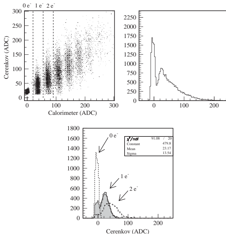
Fig. 21. Top left: scattered plot of the signal from the Cherenkov counter vs. the signal from the calorimeter (in ADC counts units). Top right: the raw spectrum of the Cherenkov signal. Bottom: three different spectra obtained from the same data but requiring 0,1,2 electrons in the calorimeter (the relative cuts are shown by the dashed lines in the top left of the scatter plot). When no electrons are detected in the calorimeter only pedestal is measured at the Cherenkov (dotted line histogram). When a single electron is detected in the calorimeter, the peak relative to one electron is clearly visible also in the Cherenkov (shaded histogram) even if the part of the signal overlapping with the no electrons position reveals some inefficiency in the detector due mainly to its small acceptance, the broader peak in the Cherenkov spectrum (dashed line histogram) corresponds to two electrons in the calorimeter.
