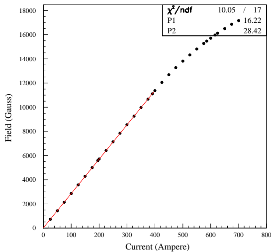
Fig. 6. Excitation curve for Dipole 1 magnet.
