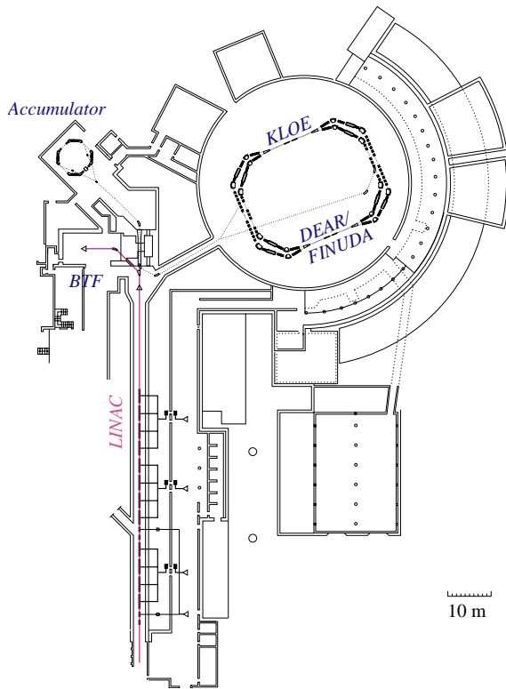
Fig. 1. Layout of the DAΦNE complex showing the LINAC, the Accumulator, the Main Rings and the Beam Test Facility (BTF).
