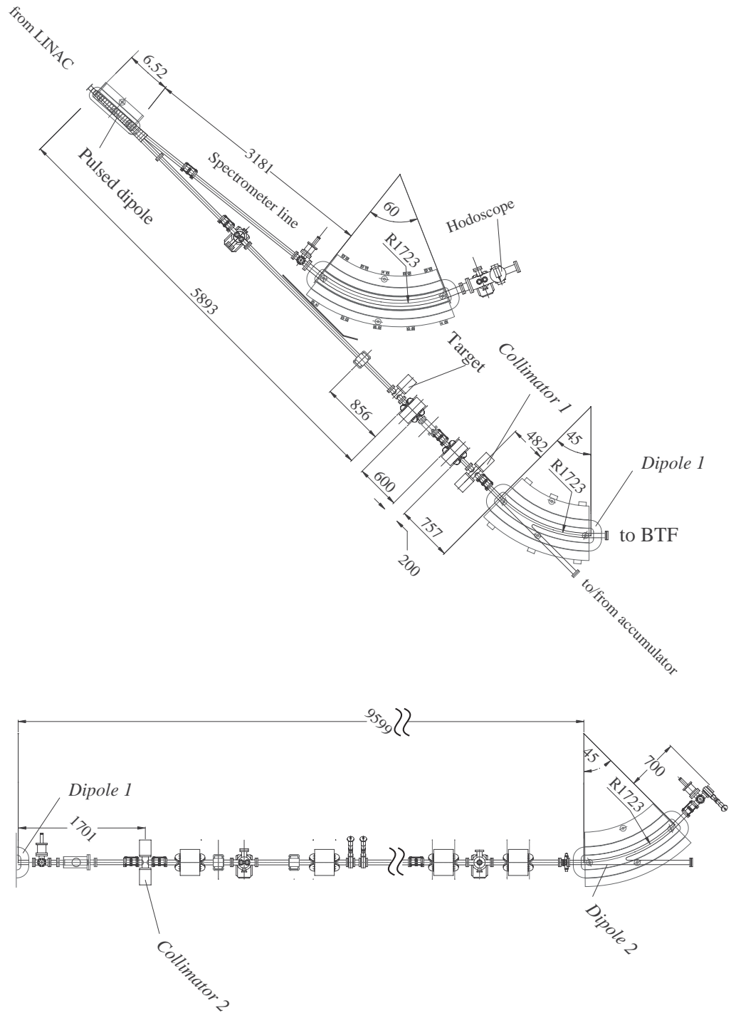
Fig. 2. The BTF transferline. Top: the first part of the line from the LINAC to the energy selector magnet ( Dipole 1 ) is shown with its main elements: the pulsed magnet sending one pulse out of 50 (25) into the LINAC spectrometer system (dipole and hodoscope), the energy degrader target and the Collimator 1 before the energy selector magnet. Bottom: the transferline to the BTF hall where two beam output ports can be selected by Dipole 2 .
