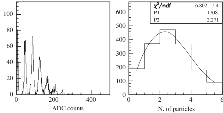
Fig. 12. Counting electrons in Calorimeter 2 ( E_{\text{sel}} = 471 MeV, HV = 1 kV): charge spectrum (left), and Poisson fit of the average number of particles in each peak (right).
