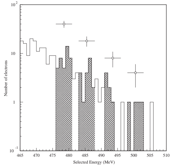
Fig. 9. Integrating the energy distribution of electrons emerging from the target (for 1.7X_0 depth) over 1% slices (shaded area), the expected number of particles as a function of the selected energy (open points) can be estimated from the Monte Carlo.
