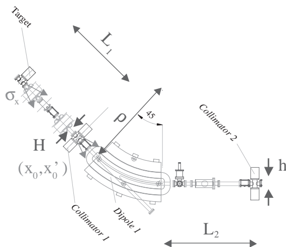
Fig. 5. Definition of the quantities relevant for the energy selector resolution: radius of curvature of the dipole, slit apertures and distances.
