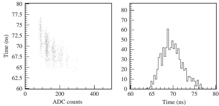
Fig. 14. Counting electrons in Calorimeter 2 ( E_{\text{sel}} = 471 MeV, HV = 1 kV): time vs. charge distribution (left) and corresponding time spectrum (right).
