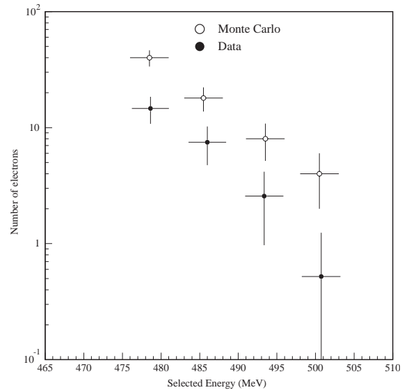
Fig. 20. Expected number of particles per bunch as a function of the selected energy. The Monte Carlo calculation (empty dots) is compared with the experimental data (full dots). The target thickness was 1.7X_0 and the energy acceptance was 1%.
