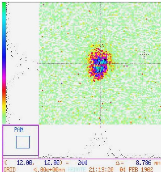
Fig. 10. High-fluorescence target image of the first beam injected into the BTF hall, on February 4, 2002.
