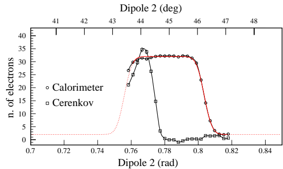
Fig. 25. Average number of electrons in the Cherenkov counter and in Calorimeter 2 as a function of the second dipole current, translated in bending angle in radians (bottom scale) and degrees (top scale), for E_{\text{sel}} = 471 MeV.
