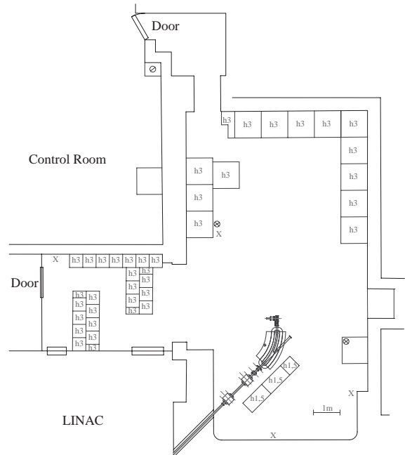
Fig. 3. Layout of the BTF experimental hall, showing the final part of the transferline with the second bending magnet ( Dipole 2). The concrete blocks of the shieldings are also shown.
