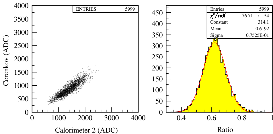
Fig. 22. Left: signal in the Cherenkov counter vs. signal in the calorimeter, in ADC counts. Right: distribution of the ratio between the two signals with the Gaussian fit used for the estimate of the average ratio. E_{sel} = 471 MeV case.
