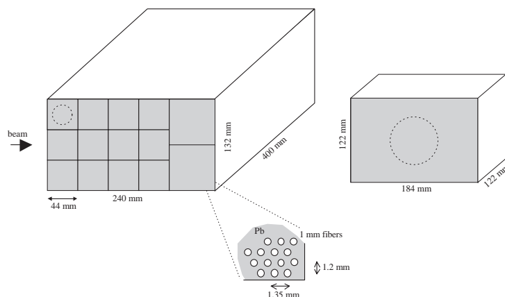
Fig. 11. Schematic view of the calorimeters: “Calorimeter 1”, the 14-cells KLOE calorimeter Prototype 0 (left); “Calorimeter 2” the single-PMT DAΦNE luminometer (right).
