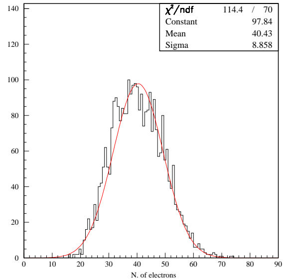
Fig. 13. The signal from Calorimeter 2 is normalized to the average deposited energy of a single electron, giving the number of particles per bunch: n = E/E_1 .
