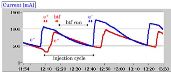
Fig. 26. Time chart of the electron and positron currents in the Main Rings showing a typical ‘parasitic’ BTF run: after the injection in the electron Main Ring the LINAC is switched for the positron injection ( \sim 3.5 min for switching); once the e^+ injection is completed the LINAC is switched to the BTF mode ( \sim 1.5 min). The BTF run lasts up to the next electron injection (3.5 min again needed to switch to e^- ). During the DEAR operation the electron beam was injected every \approx 40 min and the BTF duty cycle was about 50%.
