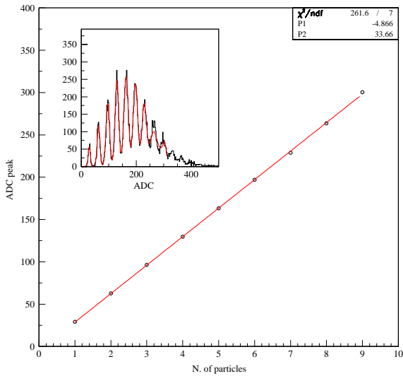
Fig. 19. Counting electrons in Calorimeter 2 ( E_{\text{sel}} = 442 MeV, HV = 1 kV): peaks linearity. Inset: a multi-Gaussian fit to the ADC spectrum.
