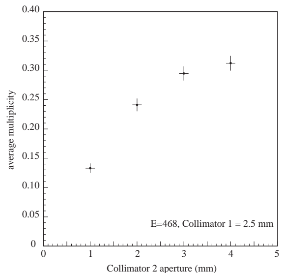
Fig. 18. Measured multiplicity as a function of Collimator 2 aperture.
