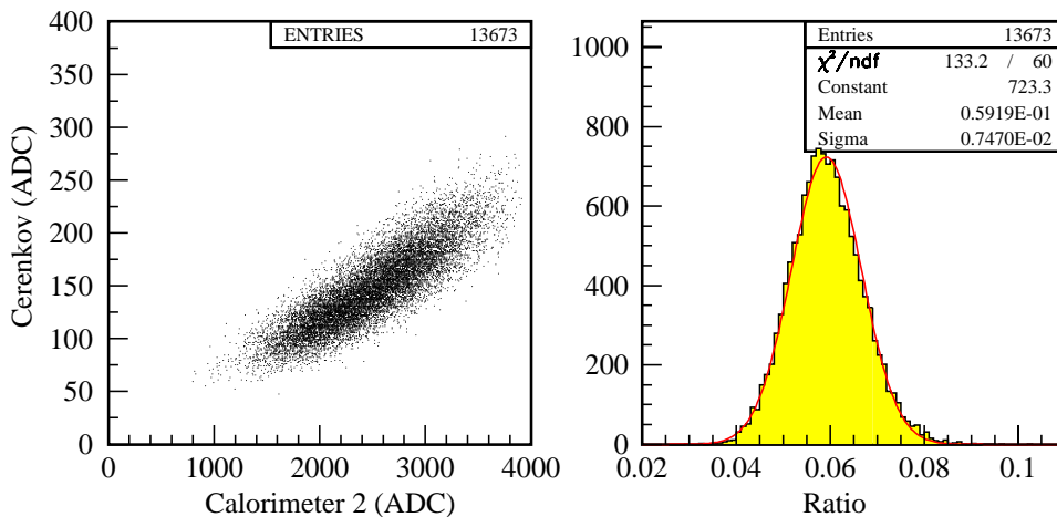
Fig. 23. Left: signal in the Cherenkov counter vs. signal in the calorimeter, in ADC counts. Right: distribution of the ratio between the two signals with Gaussian fit when an optical filter with attenuation factor = 10 is inserted between the radiator and the photomultiplier ( E_{sel} = 471 MeV). For these measurements, the beam intensity was increased by opening the downstream collimator for increasing the signal in the Cherenkov counter.
