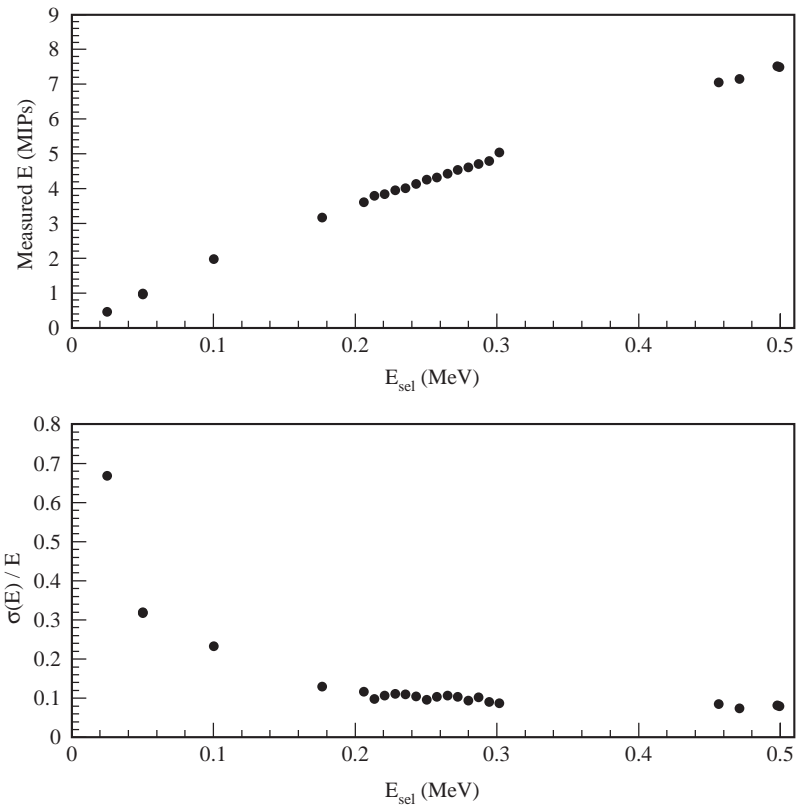
Fig. 17. Energy deposited in Calorimeter 1: the average (top) and relative width (bottom) of the Gaussian fit to the first electron peak is shown as a function of E_{sel} (calculated on the basis of the bending magnet setting).
