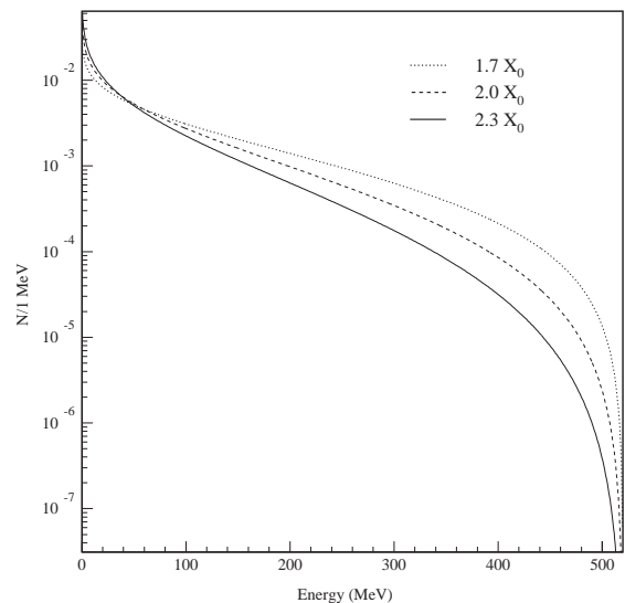
Fig. 7. Electron energy distributions out of a 1.7, 2.0, 2.3 X_0 target, calculated according to the Rossi formula of Eq. (4).
